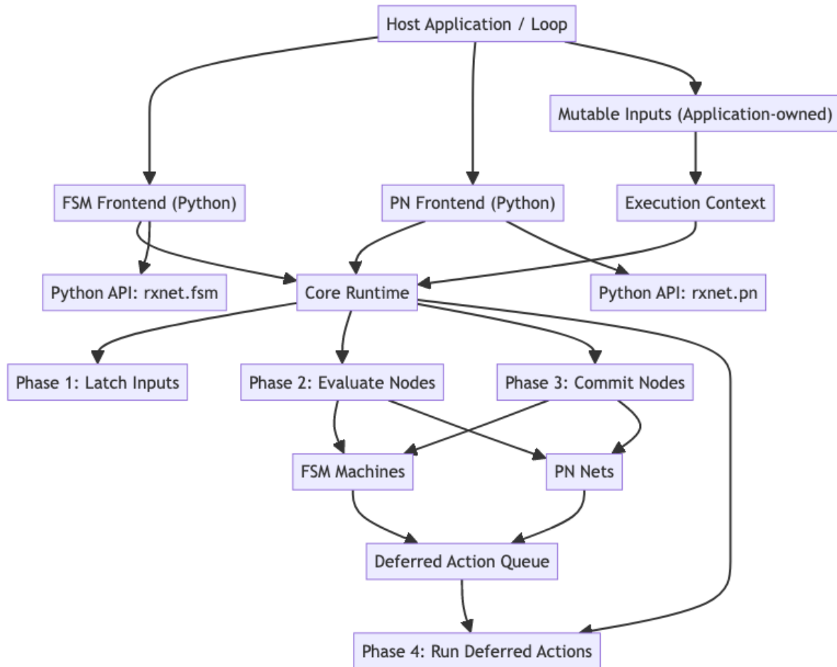
Figure 1: High-level architecture of the rxnet Python runtime and model frontends
