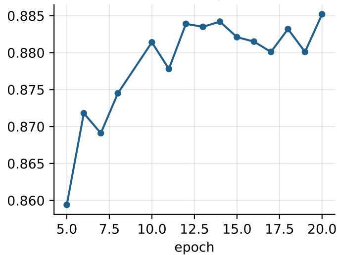
NMI (HDBSCAN, epochs 5-20)
