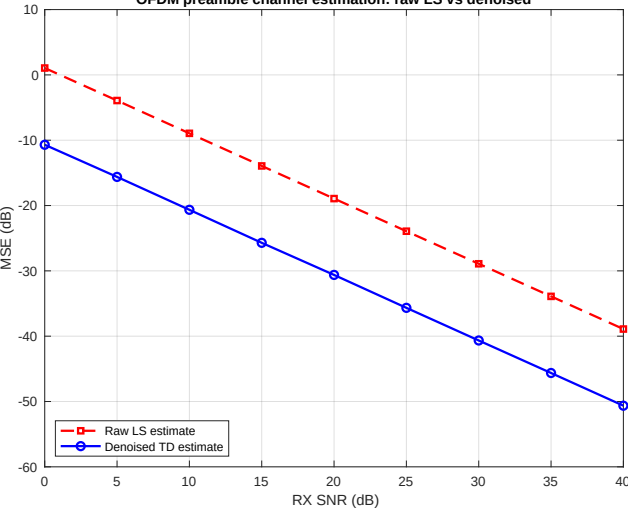
OFDM preamble channel estimation: raw LS vs denoised
