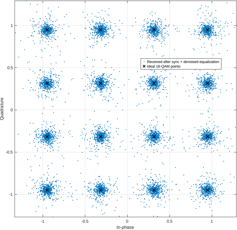
Synchronized received QAM constellation - RX SNR = 25 dB
