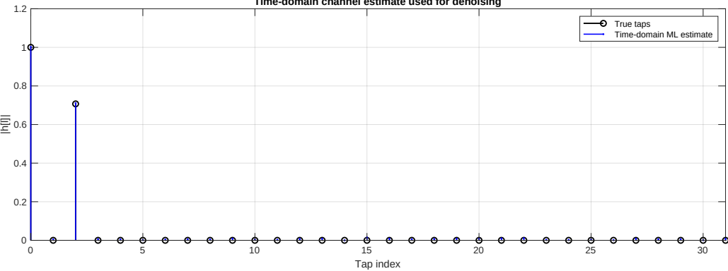
Time-domain channel estimate used for denoising
