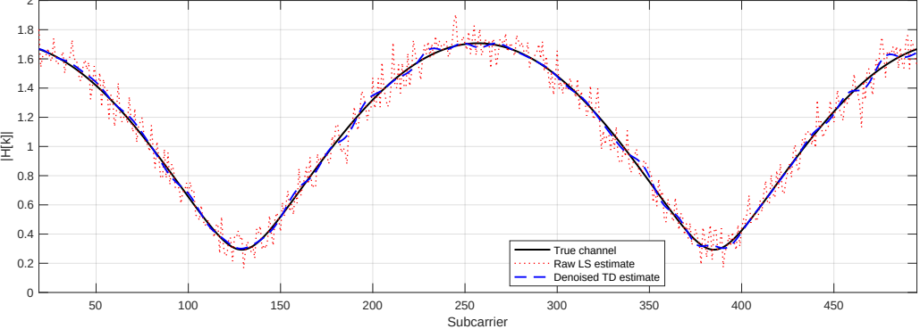
Channel estimation comparison - RX SNR = 20 dB
