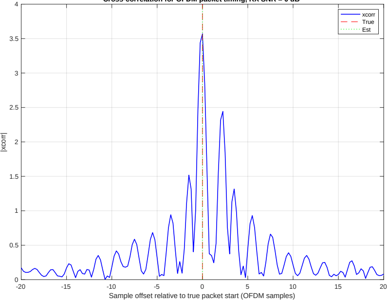
Cross-correlation for OFDM packet timing, RX SNR = 0 dB
