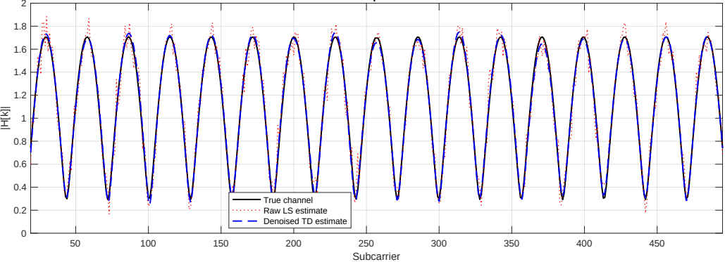
Channel estimation comparison - RX SNR = 20 dB
