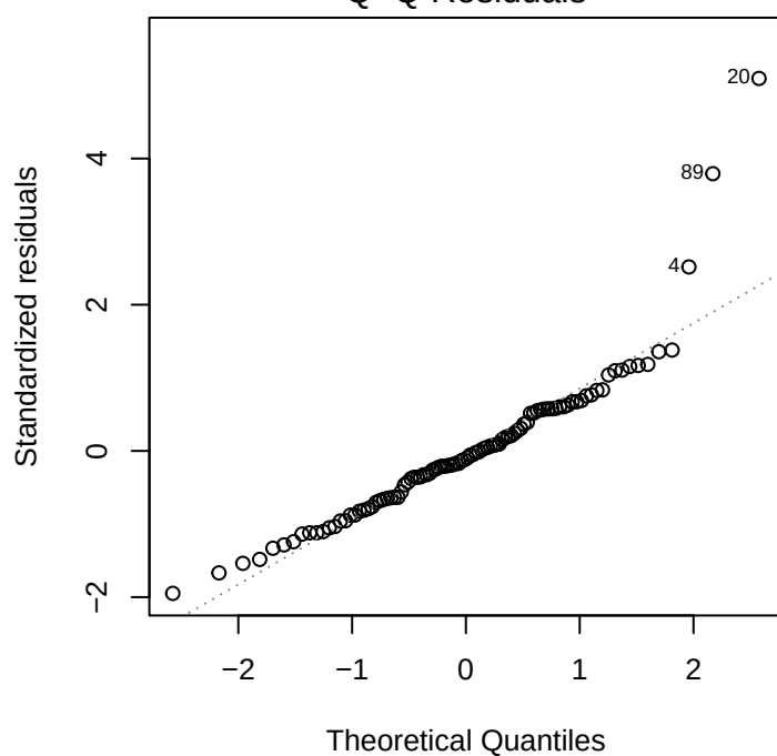
Q-Q Residuals
