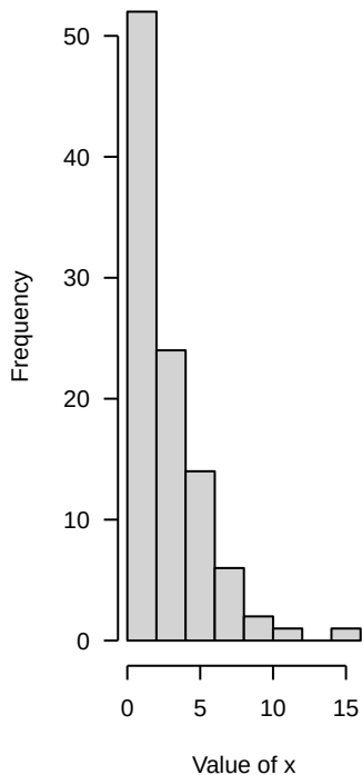
Lognormal dist.
