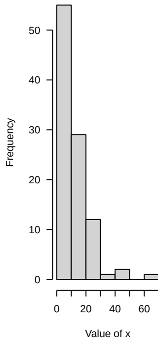
Gamma dist.
