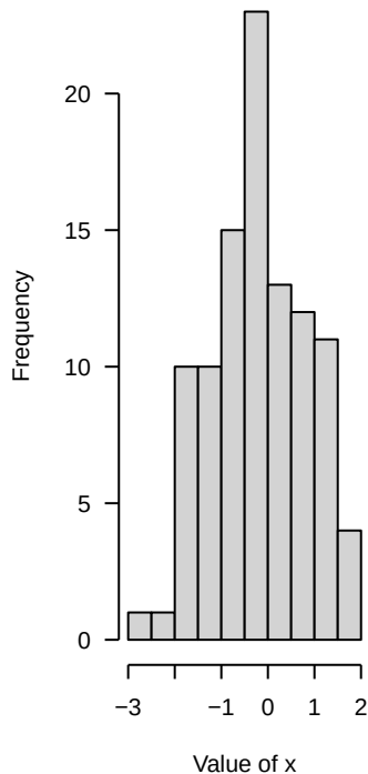
Normal dist.
