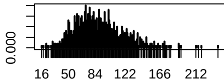
Empirical PMF
