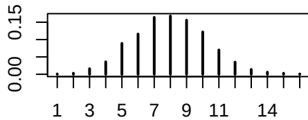
Empirical PMF
