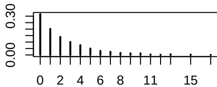
Empirical PMF
