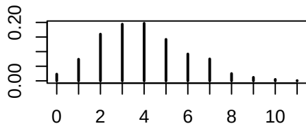
Empirical PMF
