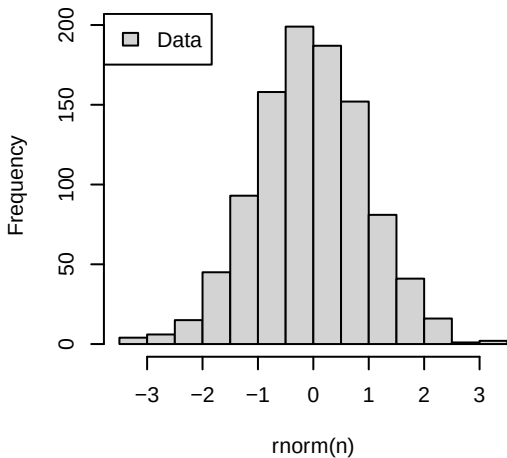
Histogram of rnorm(n)
