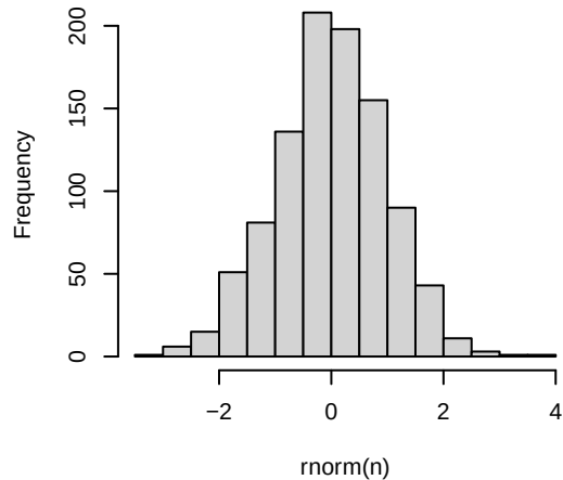
Histogram of rnorm(n)
