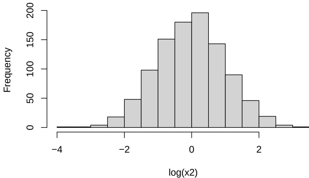
Histogram of \log(x^2)
