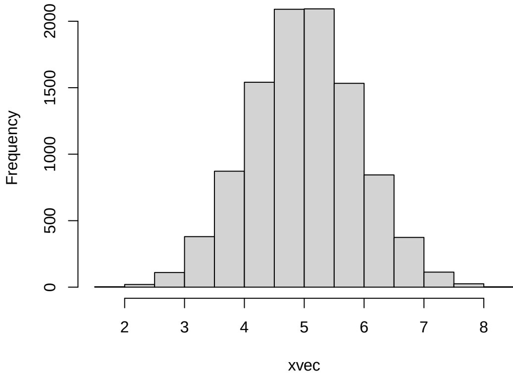
Histogram of xvec
