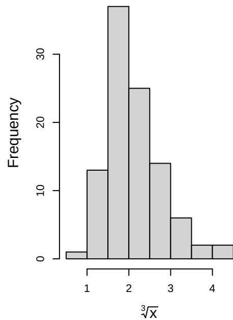
Cube root transform
