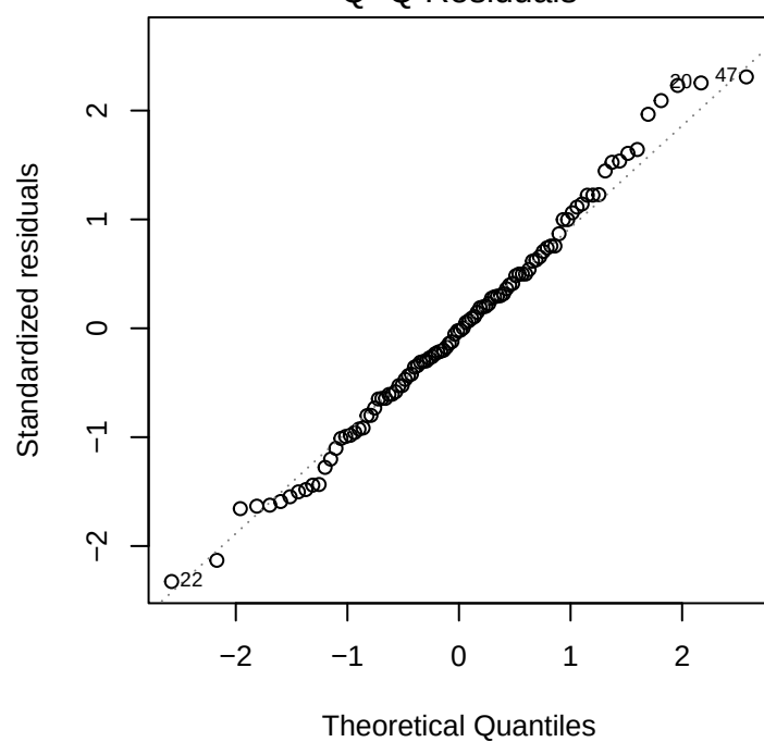
Q-Q Residuals
