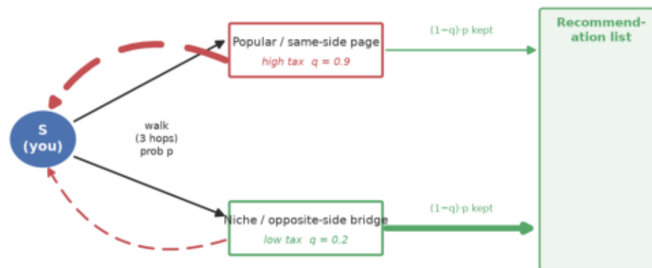
Random Walk with Erasure: a "tax" that steers recommendations
