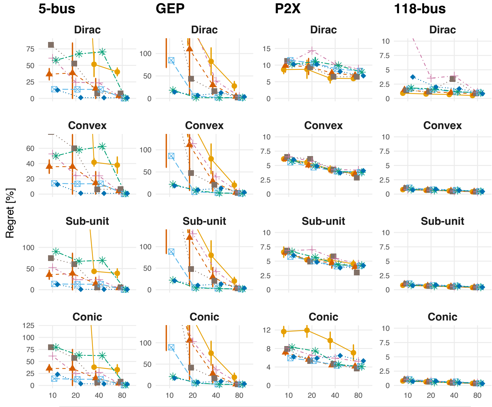
Clustering varies, conditioned on weight type
