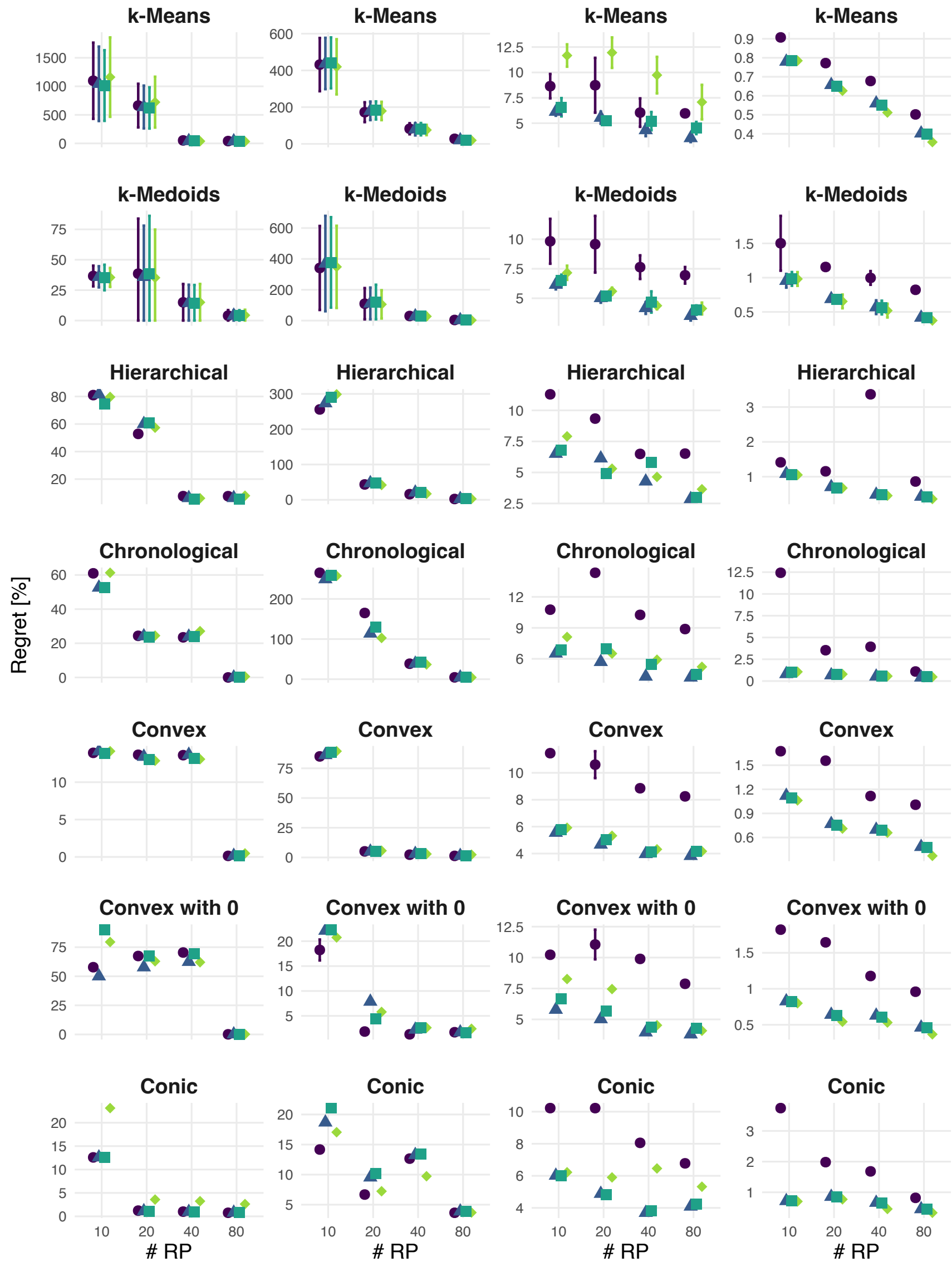
Weight type varies, conditioned on clustering method
