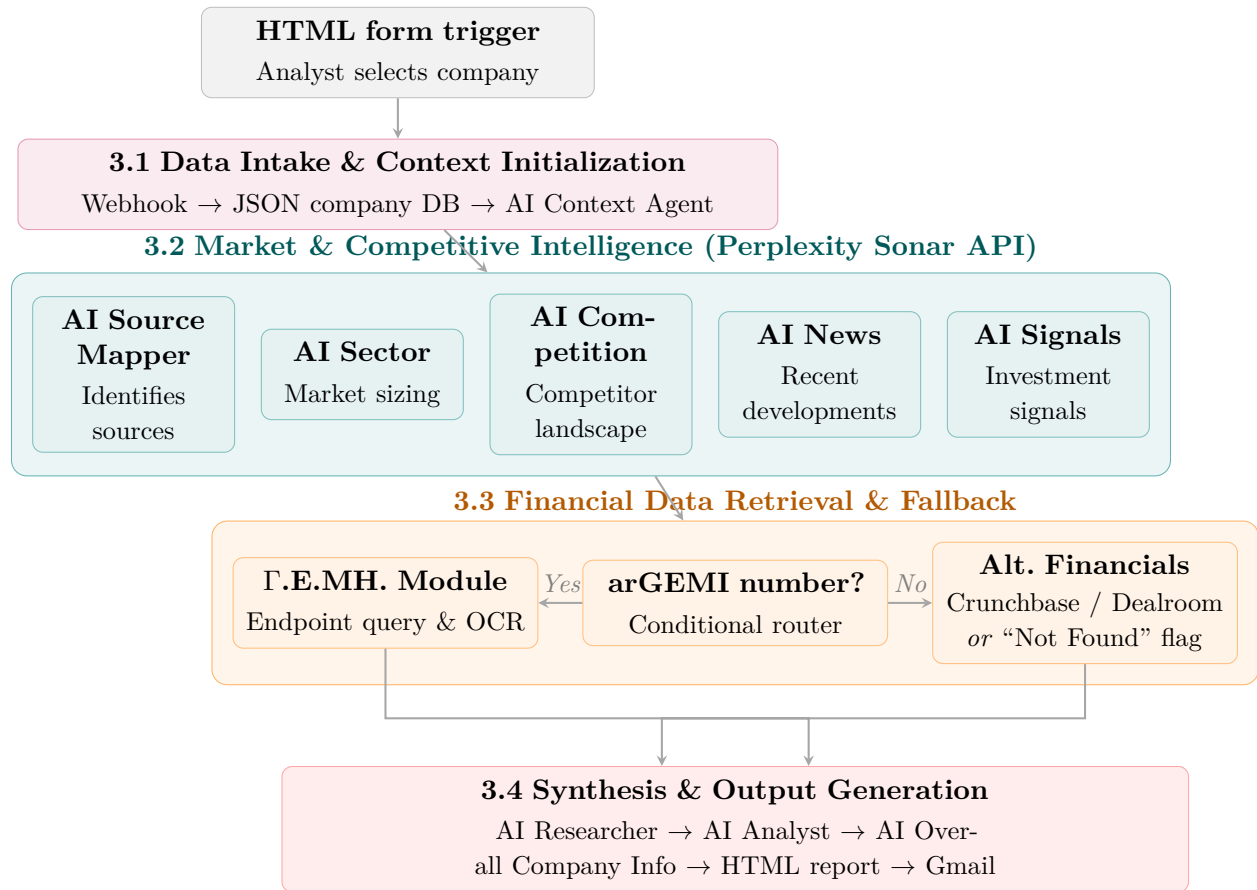
Figure 1: High-level overview of the event-driven multi-agent orchestration architecture, structured according to the four pipeline stages described in Sections 3–3.4.
