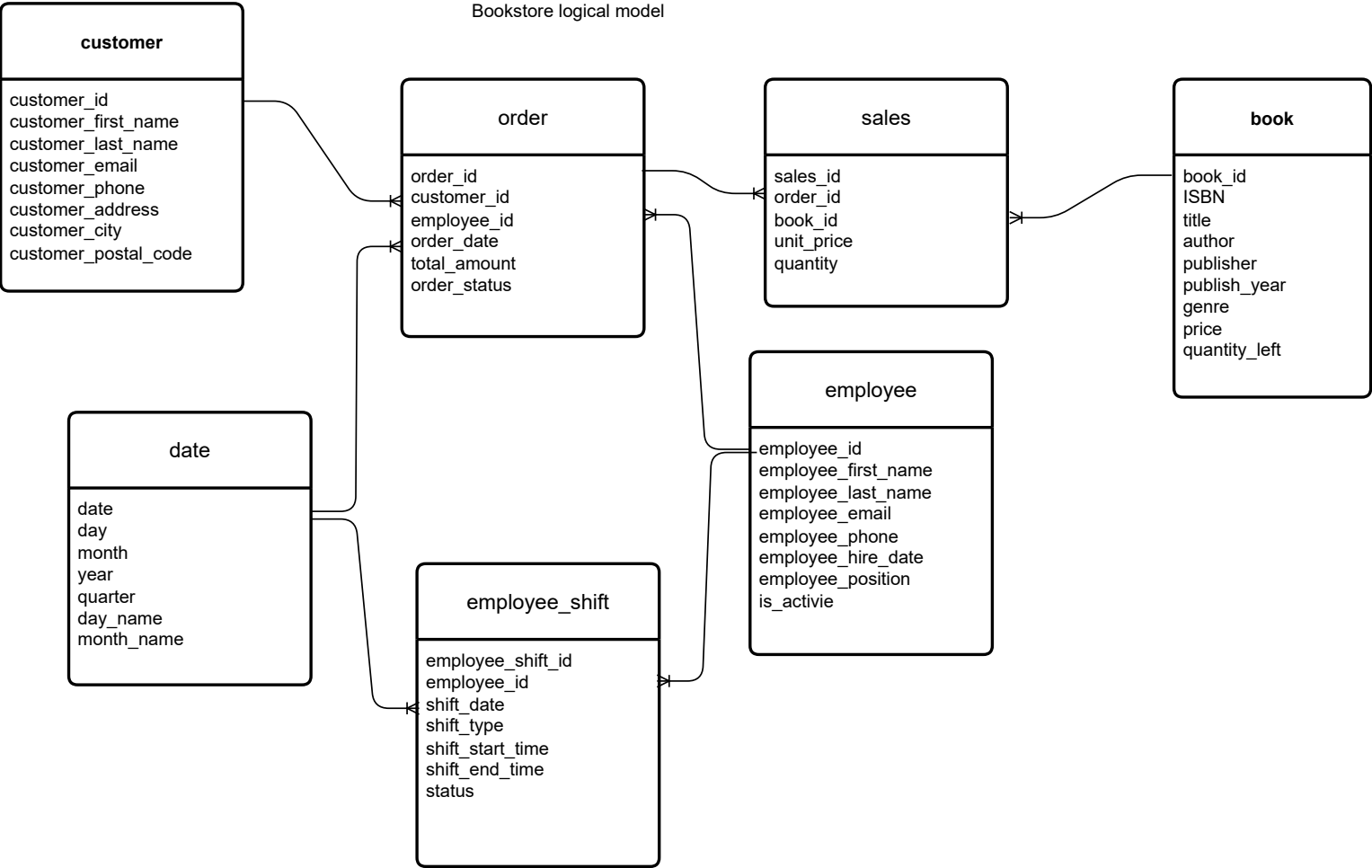
Bookstore logical model
