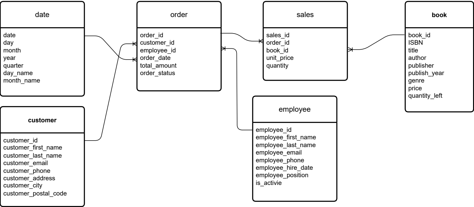
Bookstore logical model
