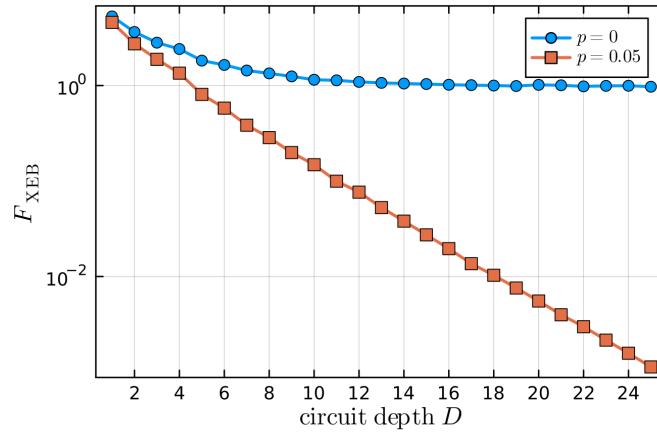
Figure 29: \mathcal{F}_{\text{XEB}} for random brick-wall circuits with N = 8 qubits as a function of the circuit depth D . The two curves correspond to the ideal case, p = 0 , and to a single-qubit depolarizing channel with error probability p = 0.05 applied after each unitary layer (see Fig. 28 ). A code example for such a simulation is given in code example #13 .
