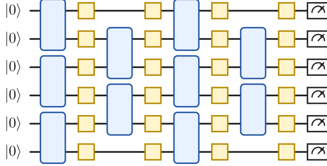
Figure 28: Brick-wall random circuit with Haar-random 2-qubit gates (blue) and single-qubit depolarizing channels (yellow), shown here for N = 6 qubits and depth D = 4 . An MPS-based code that simulates this circuit is given in code example #13 .
