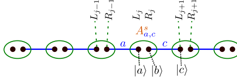
Figure 36: MPS representation of the AKLT valence-bond solid state (see also Fig. 4). The figure represents the index convention used in Eq. (108).
