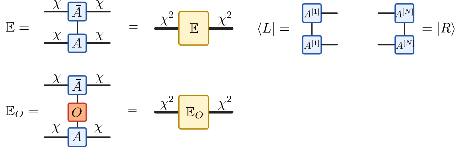
Figure 11: Graphical definition of the transfer matrix for a translationally invariant MPS. The physical index of A^s and \bar{A}^s is contracted, and the pairs of left and right virtual indices are grouped to form the matrix indices of \mathbb{E} . The second line shows the corresponding transfer matrix \mathbb{E}_O with a single-site observable inserted on the physical leg. The bottom line represents the boundary vectors \langle L| and |R\rangle used in Eq. (29).
