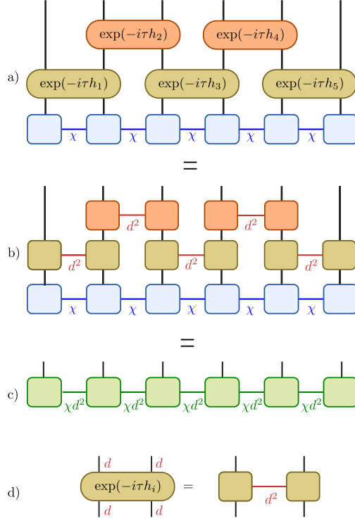
Figure 19: Time-evolution of an MPS using the TEBD algorithm. a) The time-evolution operator is decomposed into a product of two-site gates e^{-i\tau h_i} , which can be applied in parallel on the even and odd bonds. b) Using the fact that each e^{-i\tau h_i} is a two-site operator, the SVD of the associated d^2 \times d^2 matrix can be used to write it as a product of two tensors with bond dimension at most d^2 [as shown in d)]. c) After one step the MPS bond dimension has increased to (at most) \chi' = \chi d^2 . After a time step one generally needs to truncate the bond dimension of the MPS back to \chi by keeping only the \chi largest singular values.
