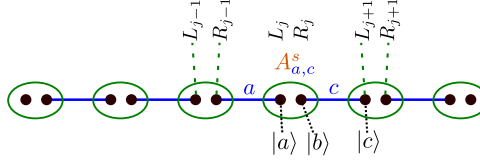
Figure 36: MPS representation of the AKLT valence-bond solid state (see also Fig. 4). The figure represents the index convention used in Eq. (108).
