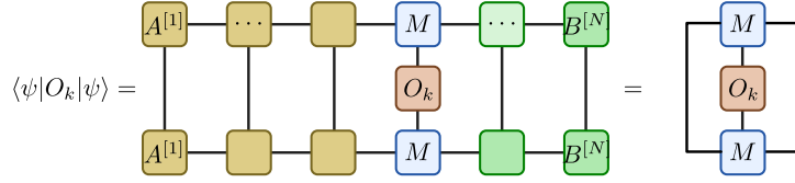
Figure 9: Expectation value of a single-site observable O at site k in an MPS written in mixed-canonical form with orthogonality center at site k . The contraction simplifies and only the tensor M at the orthogonality center remains.
