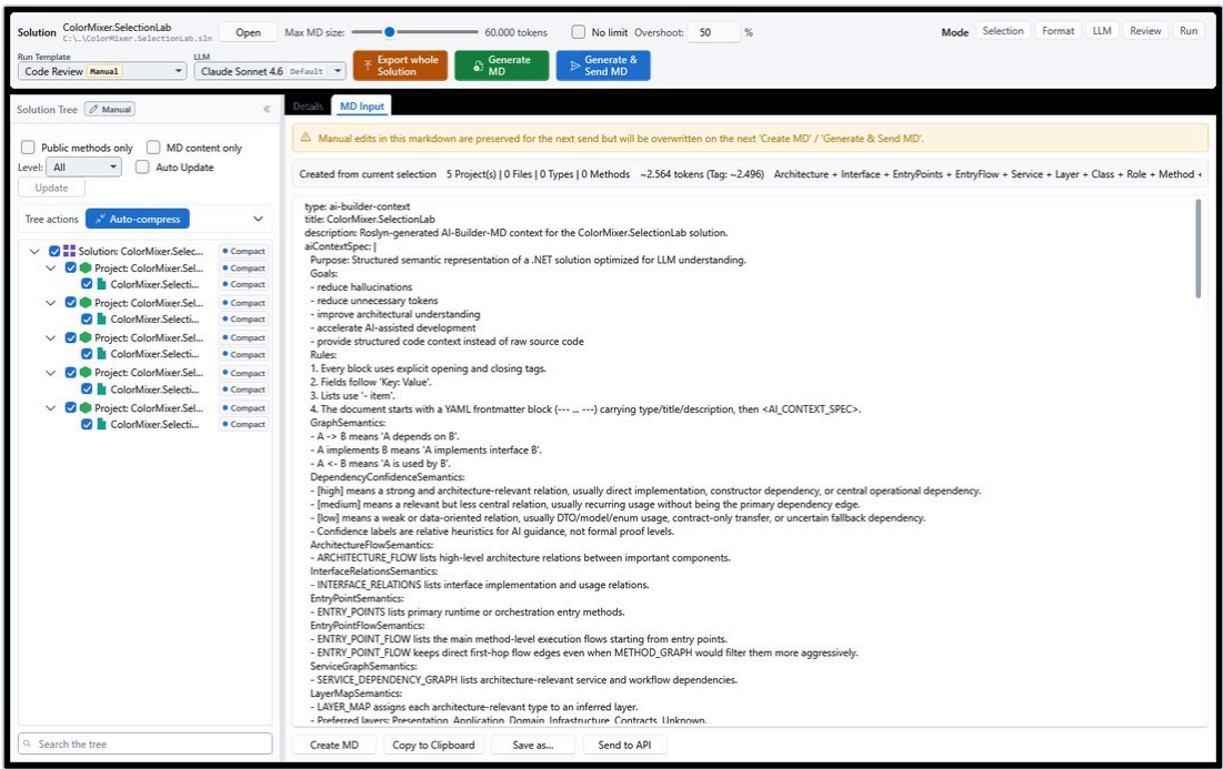
The desktop app with a solution loaded: the solution tree on the left, the generated context document on the right
