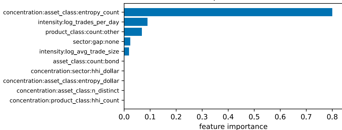
top 10 features
