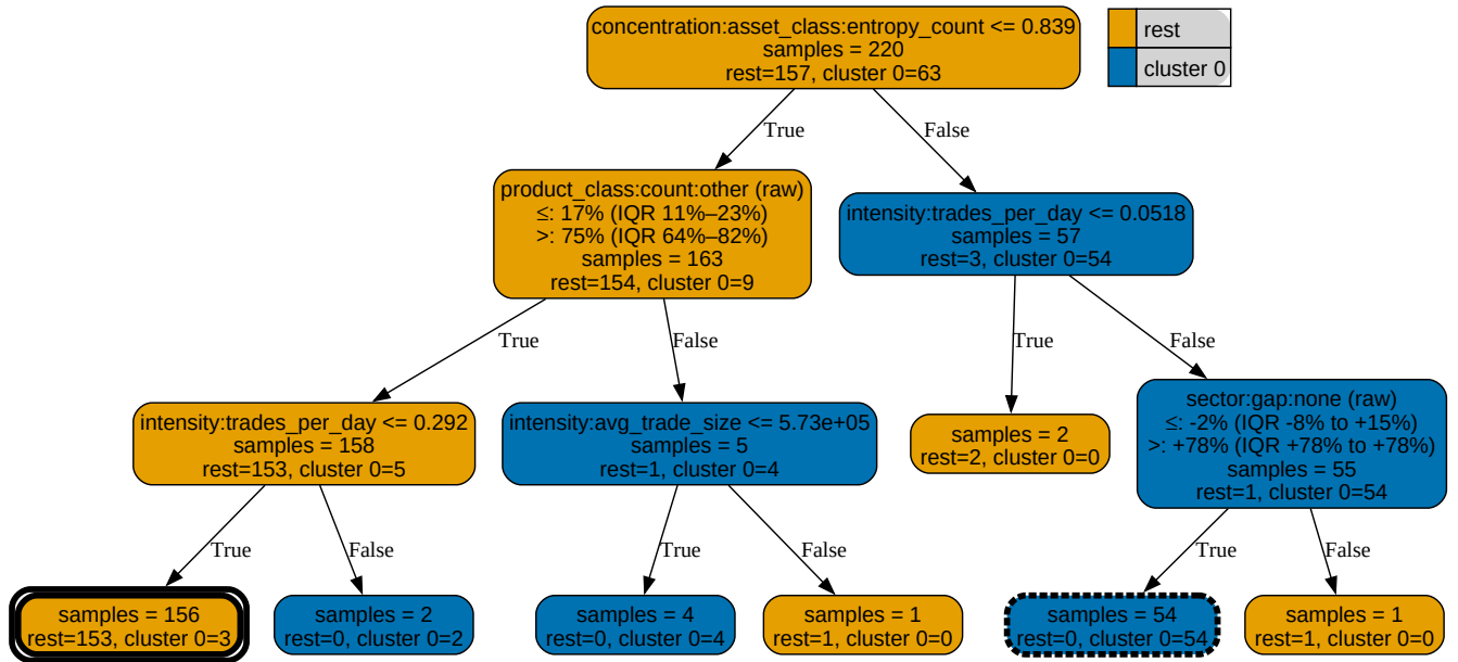
top 10 features
