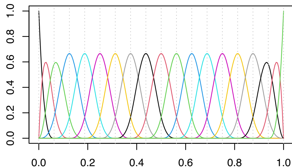
B-splines of order 3 based on 16 intervals
