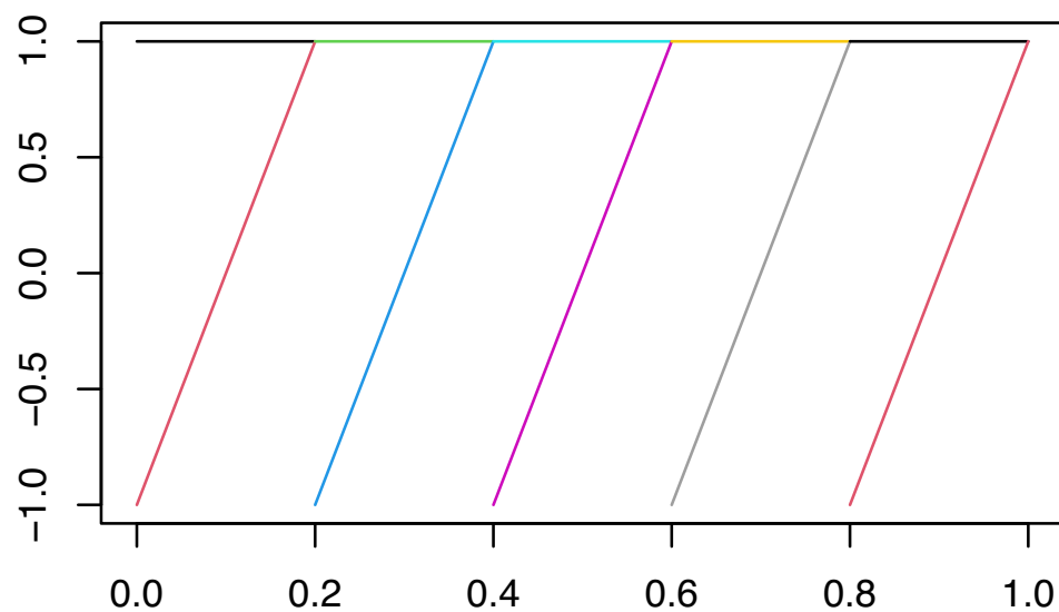
Legendre basis of order 1
