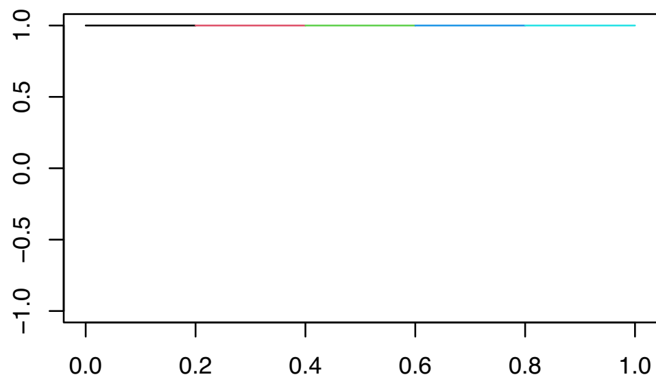
Legendre basis of order 0
