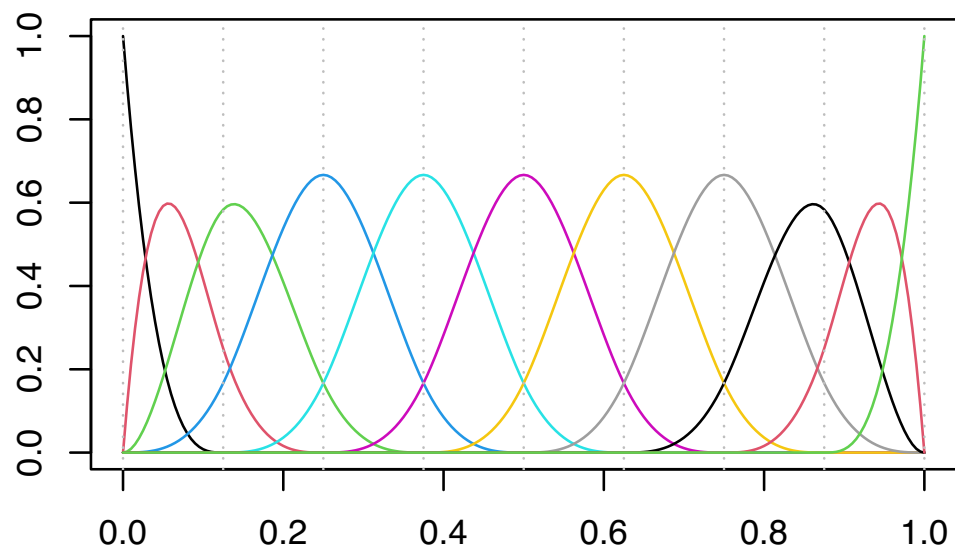
B-splines of order 3 based on 8 intervals
