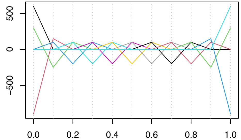
2nd derivatives of cubic B-splines
