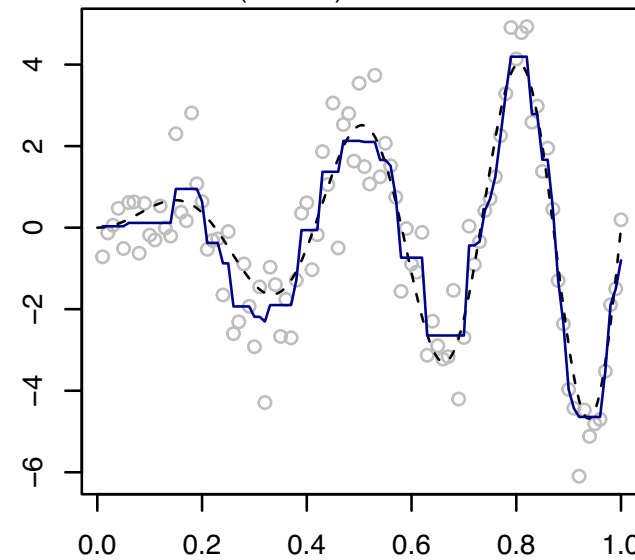
TF (order 0) with df = 99
