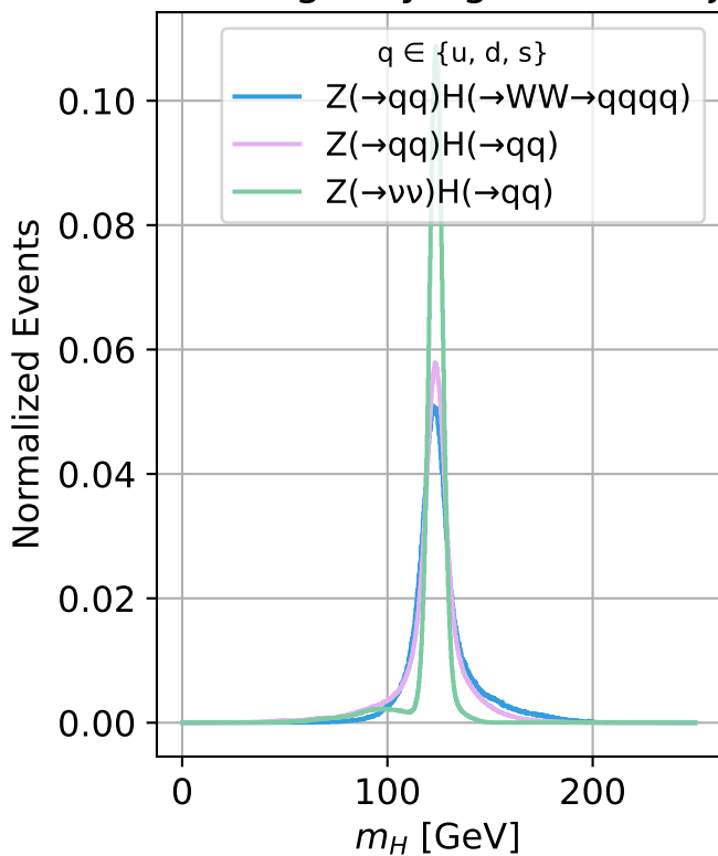
Containing only light-flavour jets
