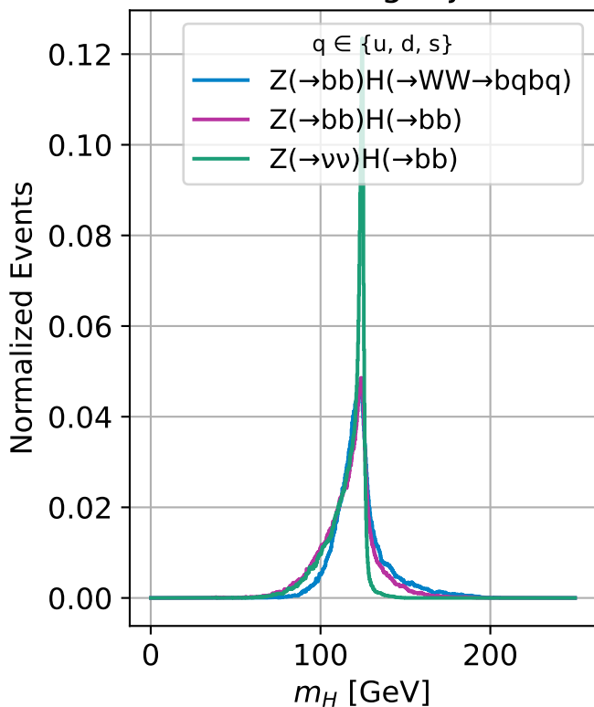
Containing b-jets
