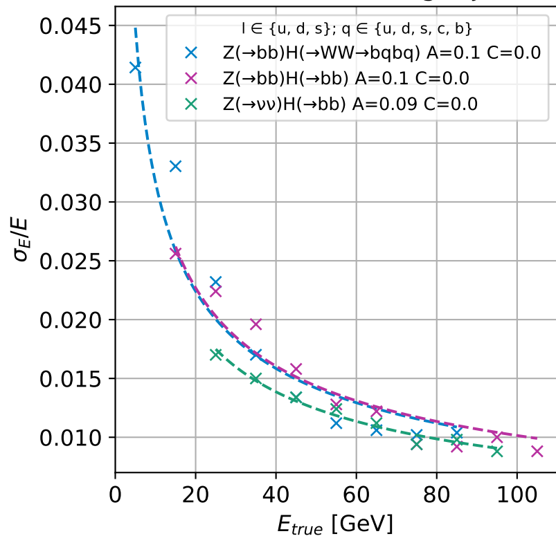
Final state containing b-jets
