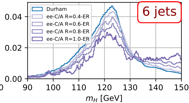
Z(\rightarrow bb)H(\rightarrow WW \rightarrow bq bq)
