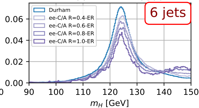
Z(\rightarrow qq)H(\rightarrow WW \rightarrow qqqq) (all f.)
