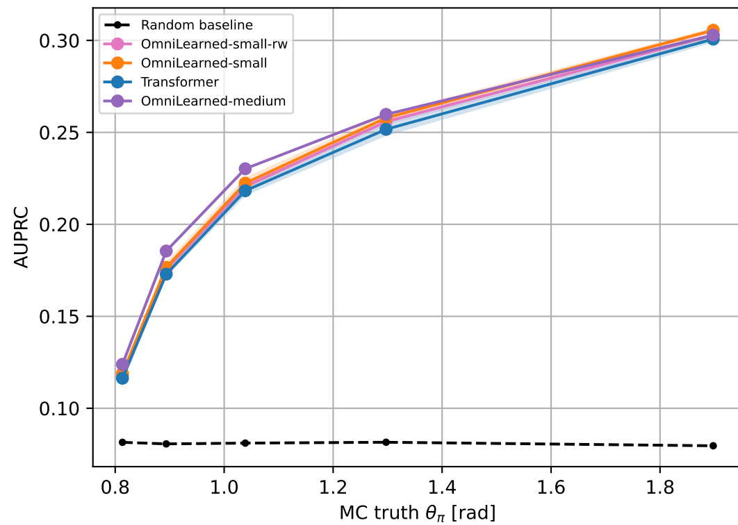
AUPRC vs. MC truth \theta_\pi
