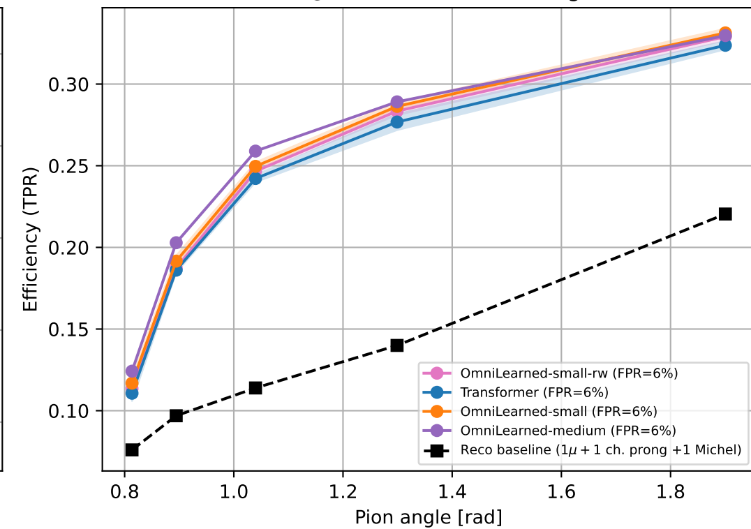
TPR @ fixed FPR vs. Pion angle
