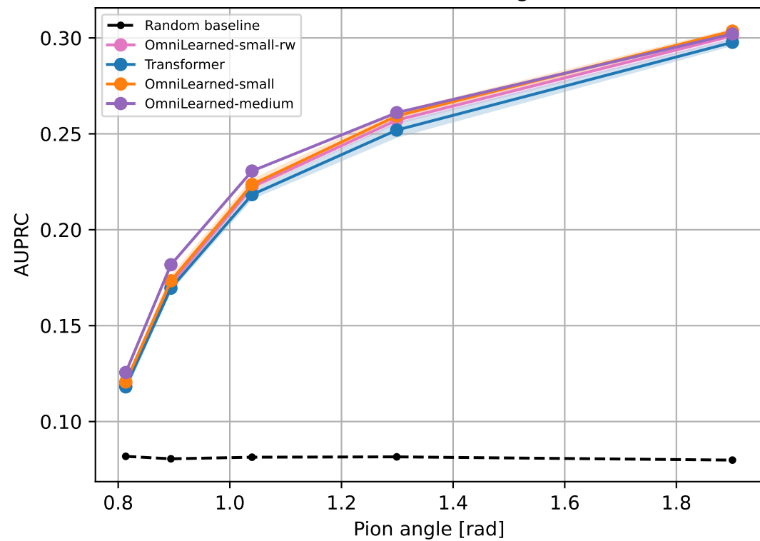
AUPRC vs. Pion angle
