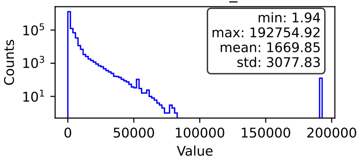
MC Particles - mc_FSPartE
