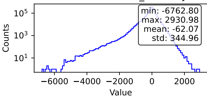
MC Particles - mc_FSPartPy
