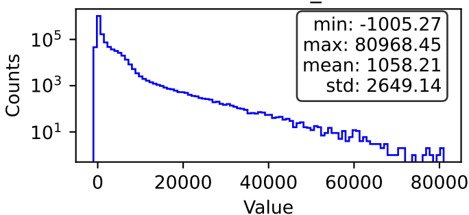
MC Particles - mc_FSPartPz
