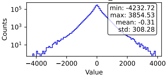
MC Particles - mc_FSPartPx
