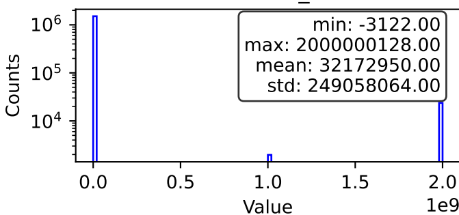
MC Particles - mc_FSPartPDG
