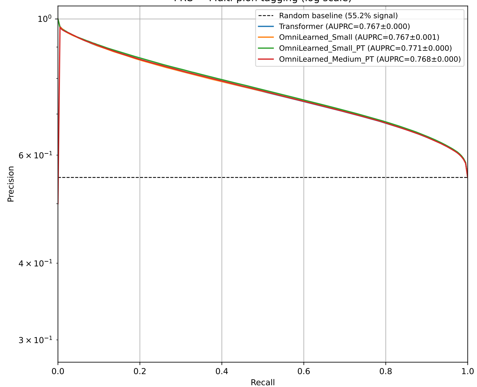
PRC — Multi-pion tagging (log scale)
