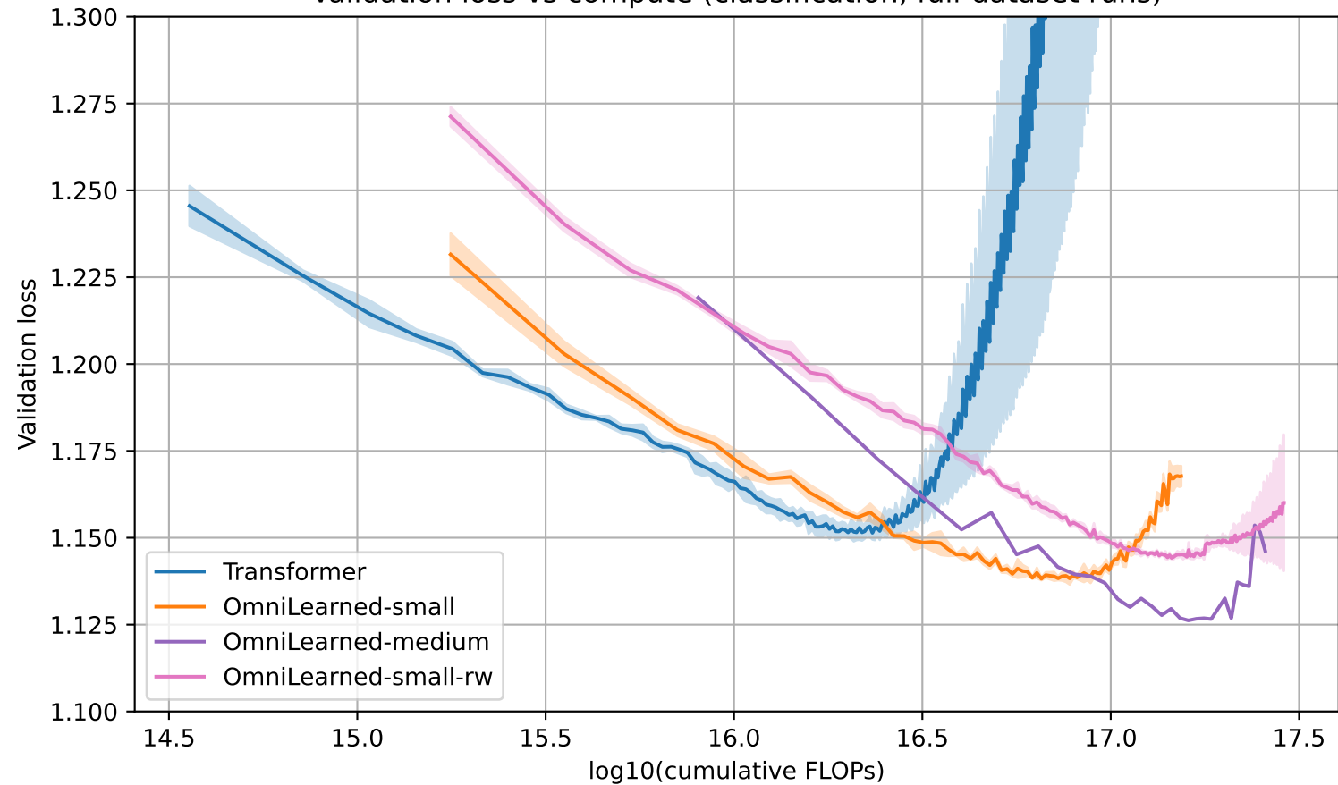
Validation loss vs compute (classification, full-dataset runs)
