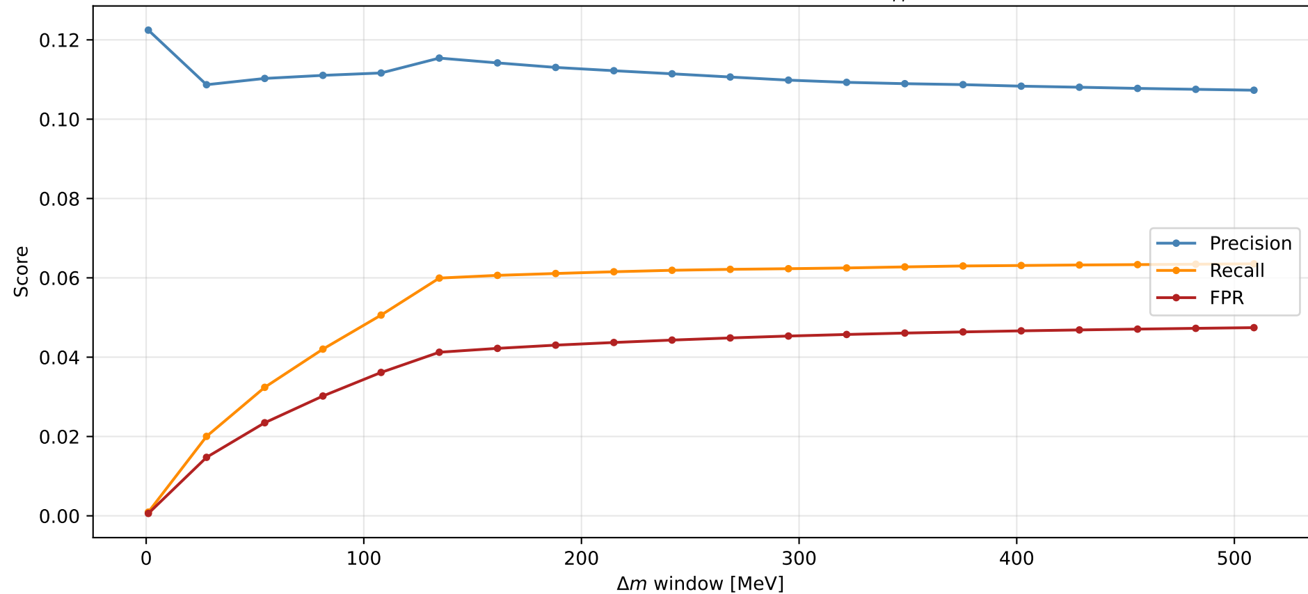
CC\pi^0 baseline: reco \mu + 2\gamma + no \pi^\pm prong + |m_{\gamma\gamma} - m_{\pi^0}| < \Delta m
