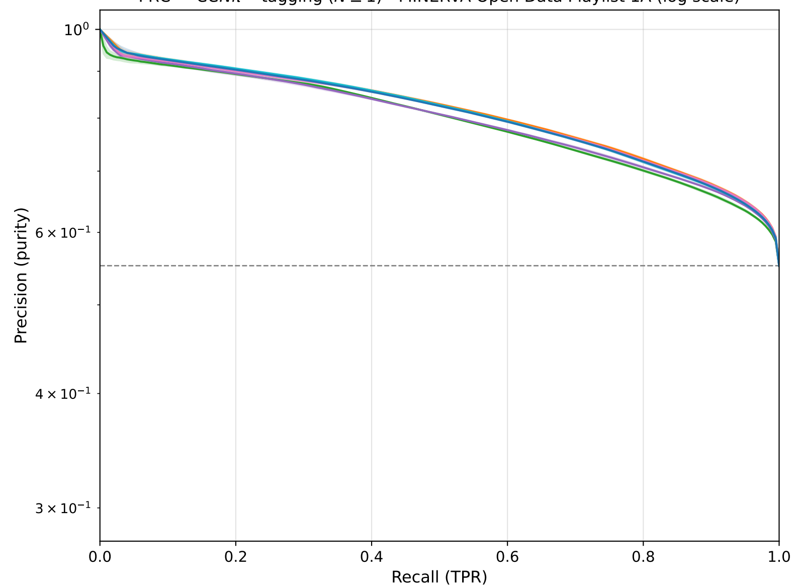
PRC — CCN\pi^\pm tagging ( N \geq 1 ) - MINERvA Open Data Playlist 1A (log scale)
