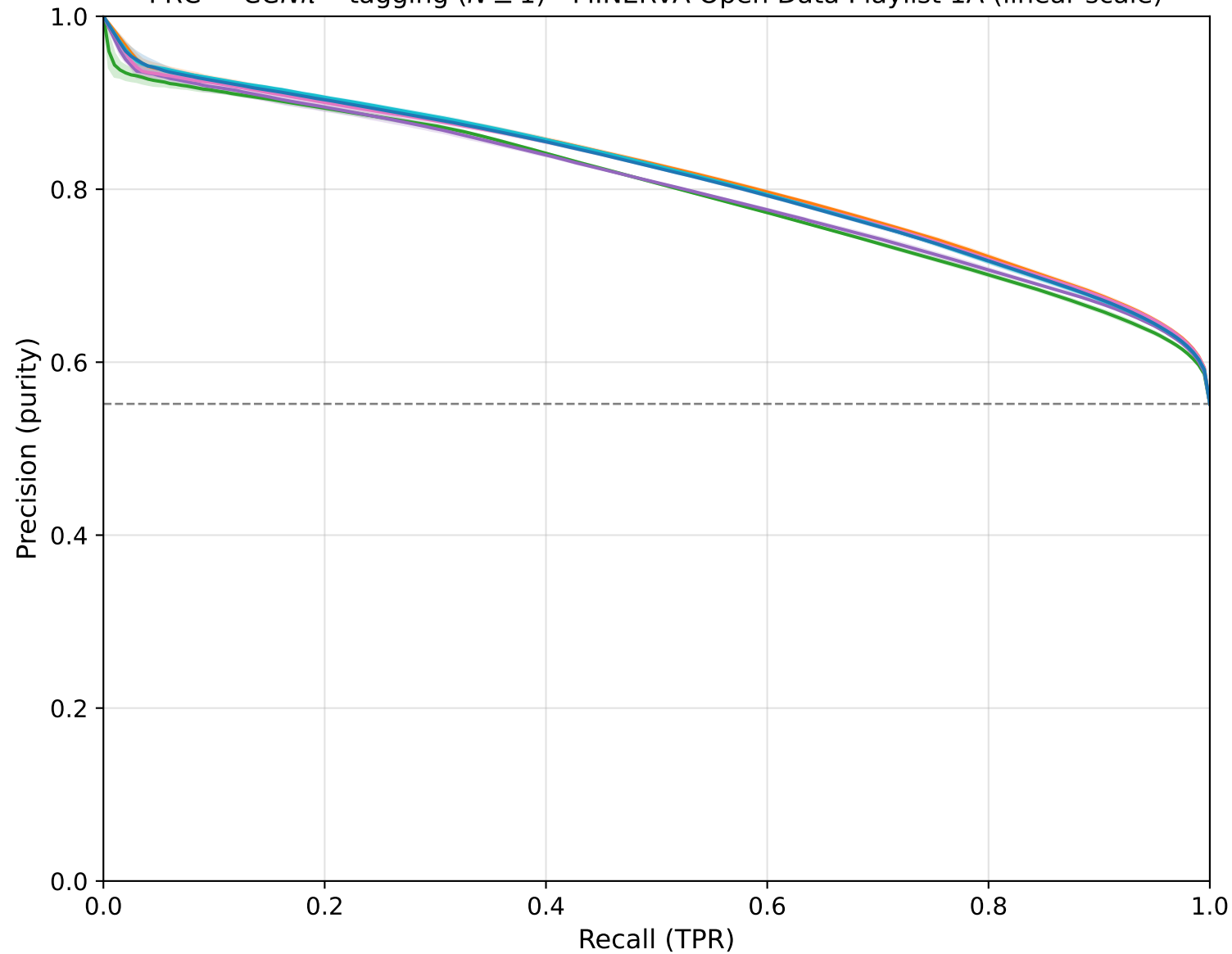
PRC — CCN\pi^\pm tagging ( N \geq 1 ) - MINERvA Open Data Playlist 1A (linear scale)
