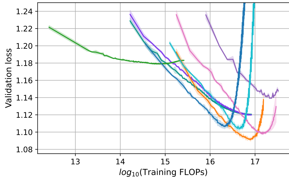
Classification
