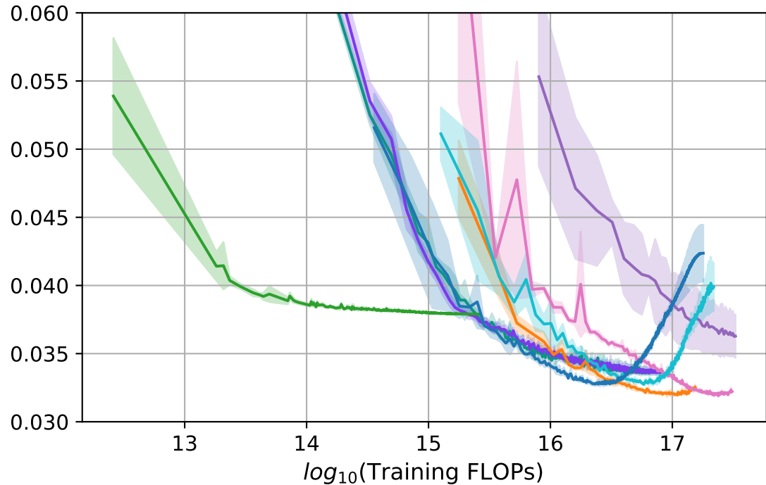
Regression
