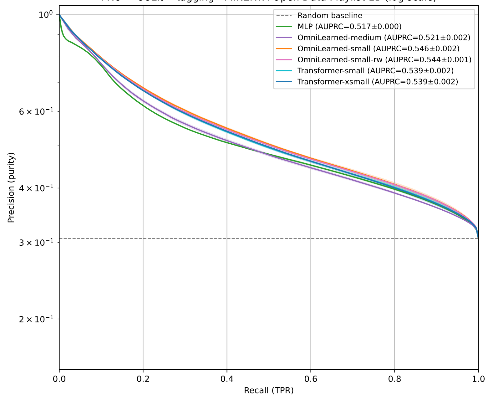
PRC — CC1\pi^\pm tagging - MINERvA Open Data Playlist 1B (log scale)
