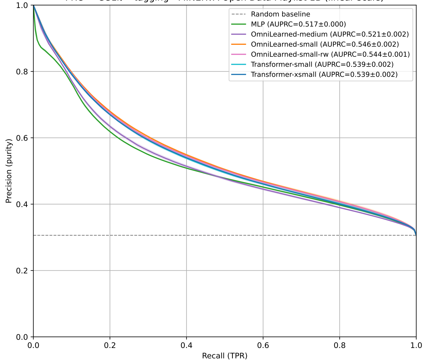
PRC — CC1\pi^\pm tagging - MINERvA Open Data Playlist 1B (linear scale)
