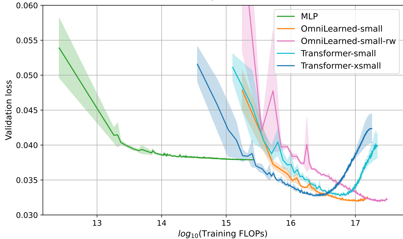
Regression
