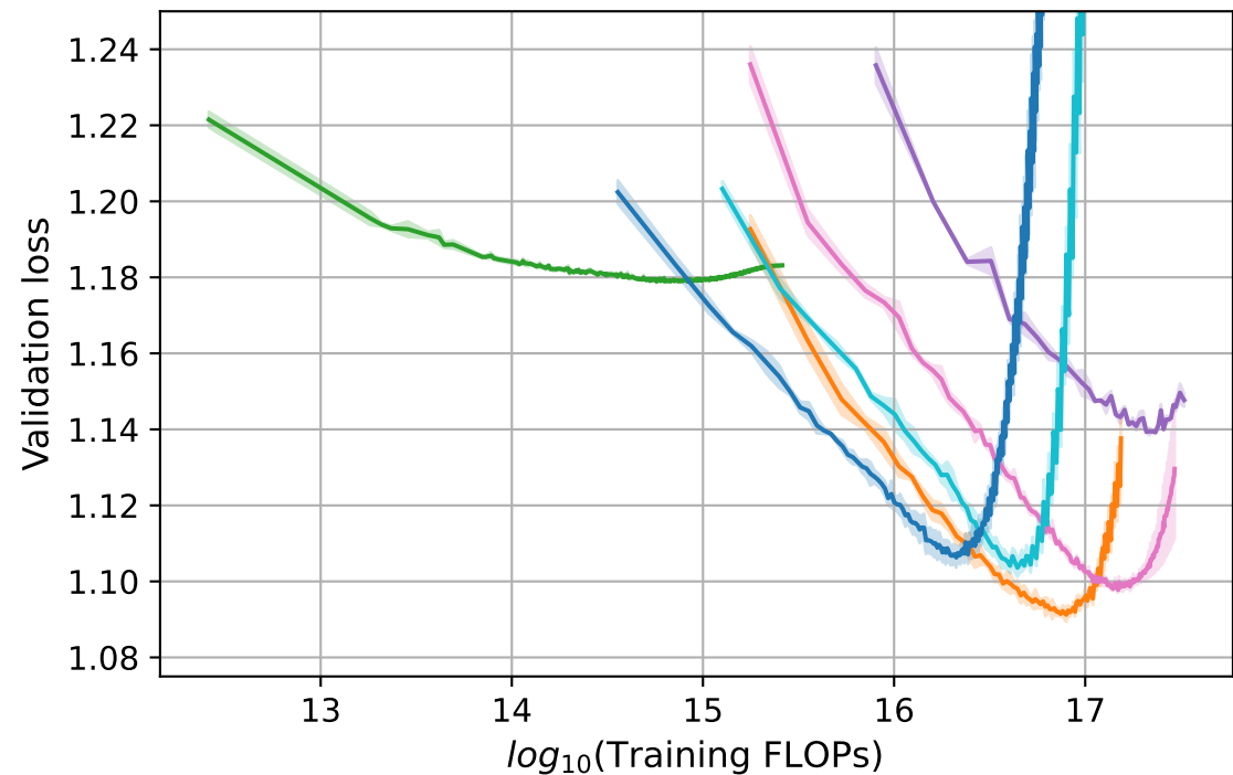
Classification
