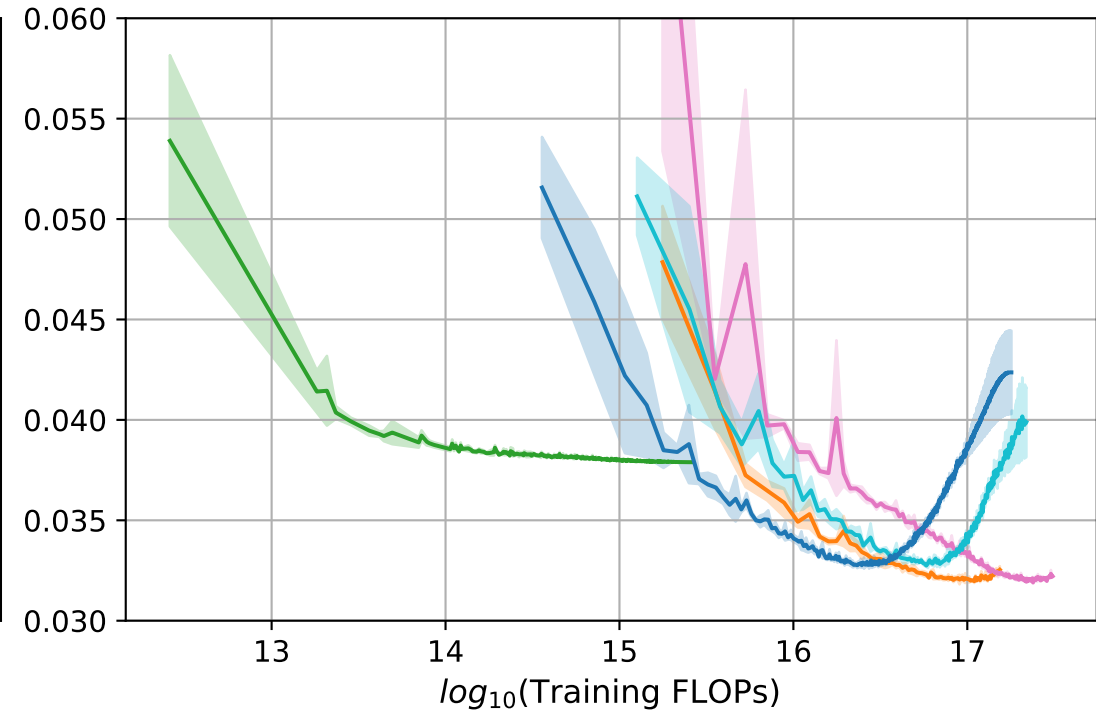
Regression
