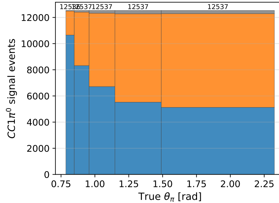
CC1\pi^0 : signal composition vs. True \theta_\pi
