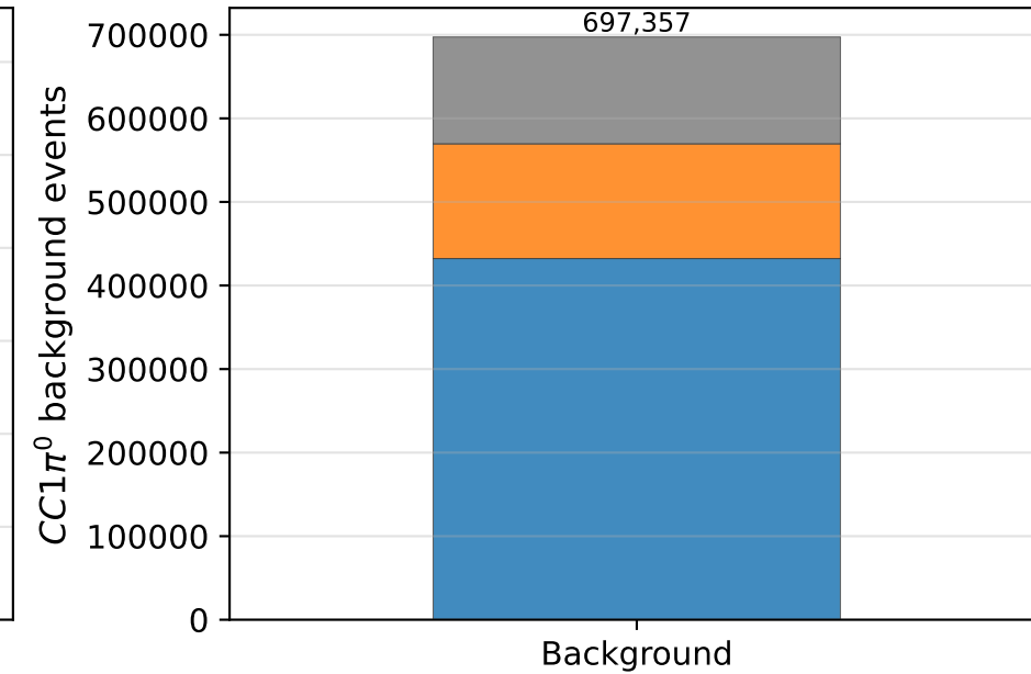
CC1\pi^0 : background composition
