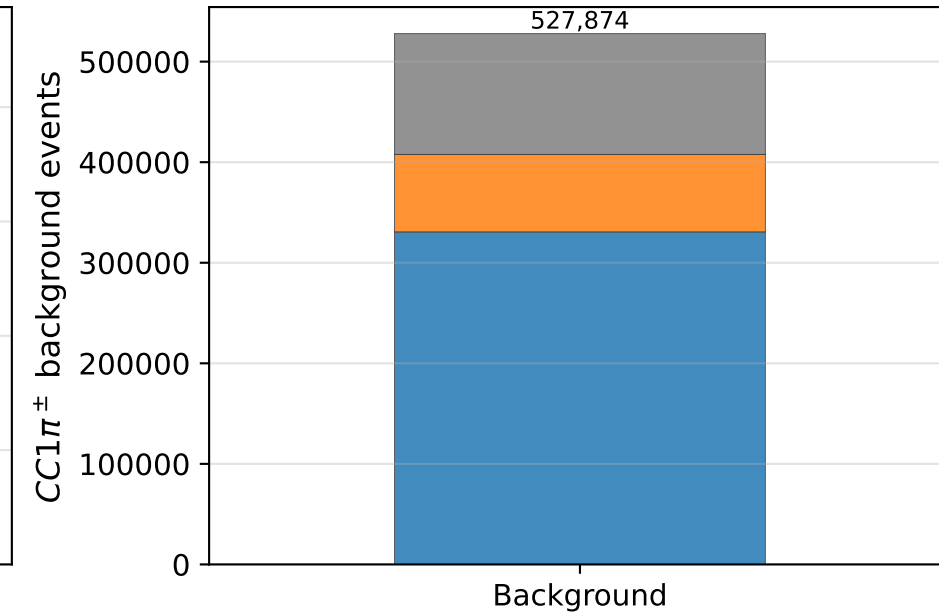
CC1\pi^\pm : background composition
