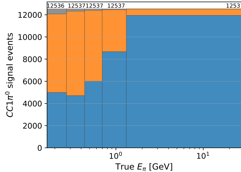
CC1\pi^0 : signal composition vs. True E_\pi
