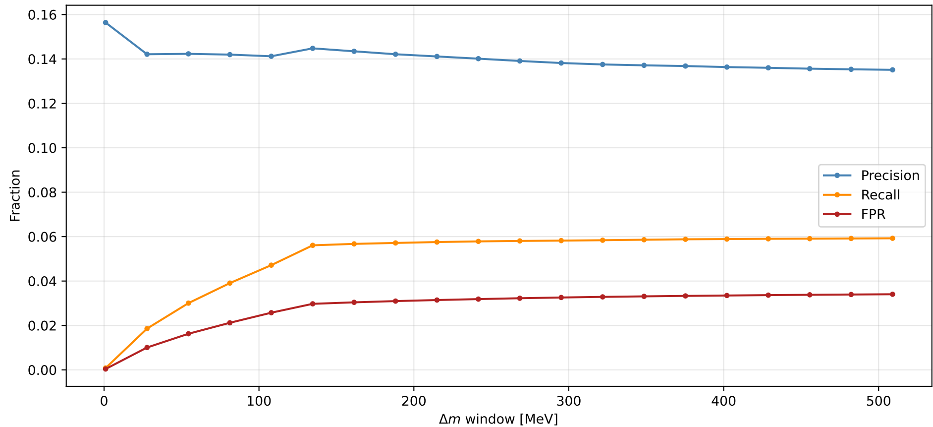
CC\pi^0 baseline vs. \Delta m window
