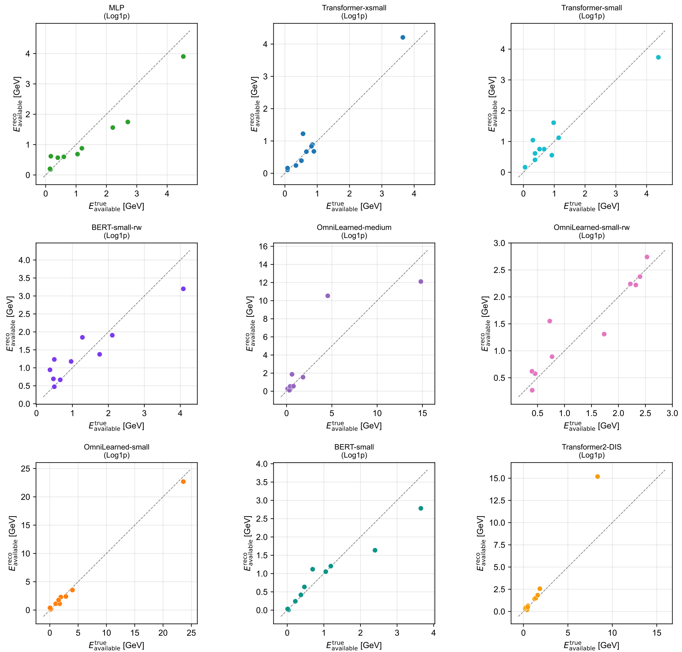
1A: 10 random selected events per method (use_cc_selection=2)
