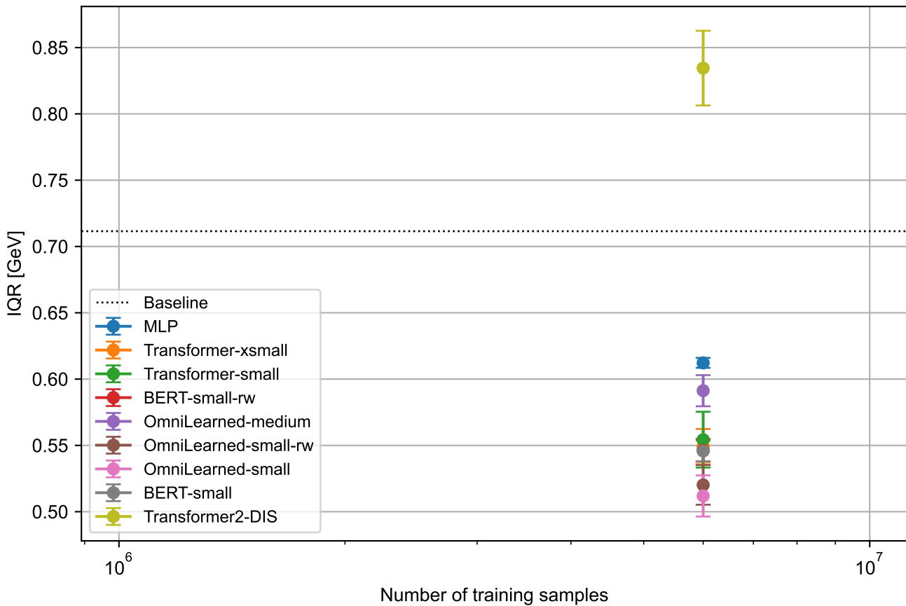
IQR vs Training Samples ( q_3 bin 2, mid = 0.90 GeV)
