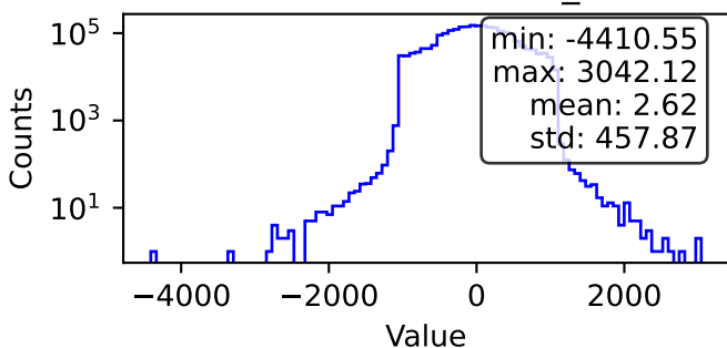
Blobs - MasterAnaDev_BlobX
