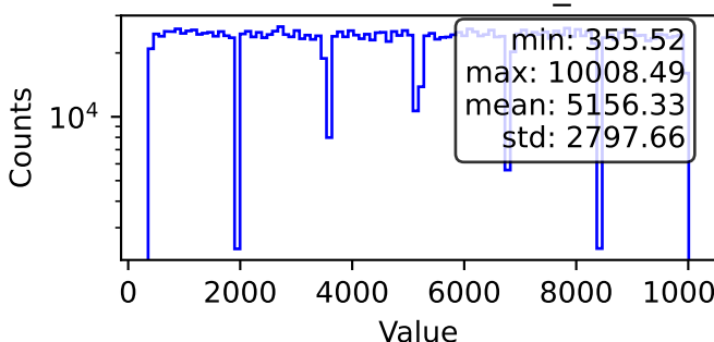
Blobs - MasterAnaDev_BlobT
