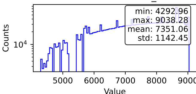
Blobs - MasterAnaDev_BlobZ
