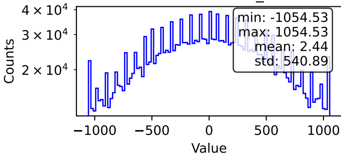
Blobs - MasterAnaDev_BlobTPos
