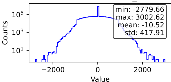
Blobs - MasterAnaDev_BlobY
