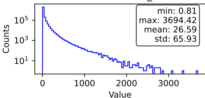
Blobs - MasterAnaDev_BlobTotalE
