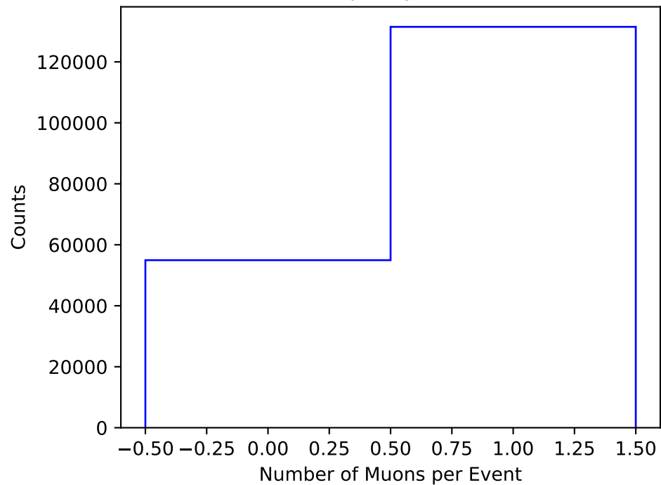
Prong Multiplicity Distribution
