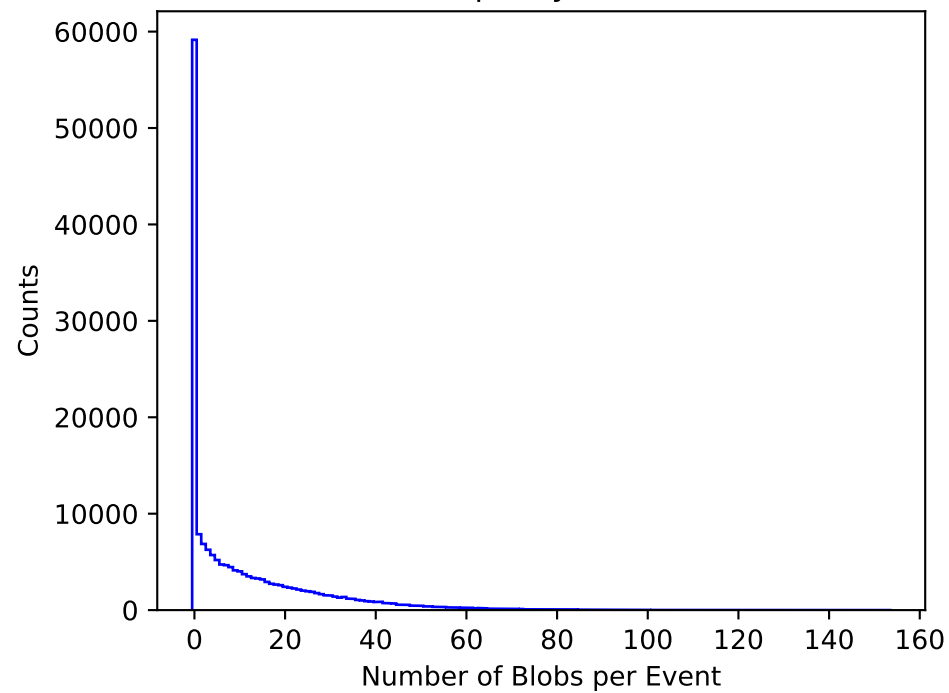
Blob Multiplicity Distribution
