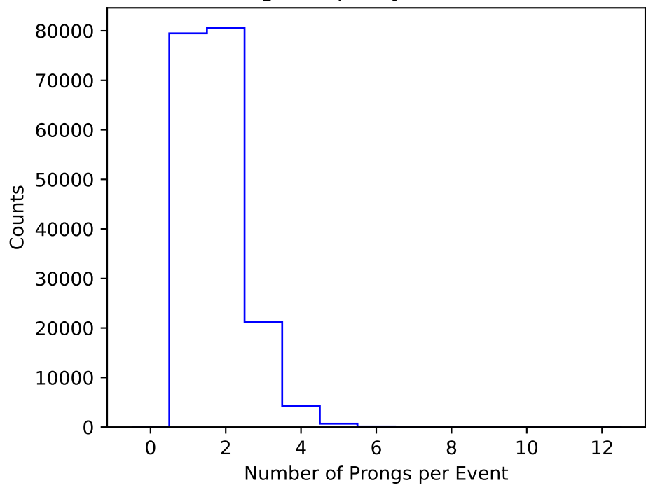
Prong Multiplicity Distribution
