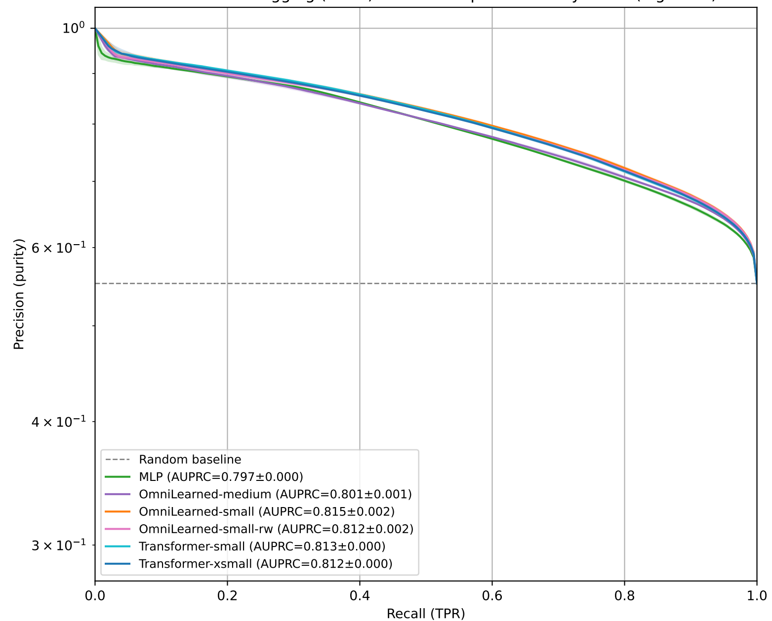
PRC — CCN\pi^\pm tagging ( N \geq 1 ) - Minerva Open Data Playlist 1A (log scale)
