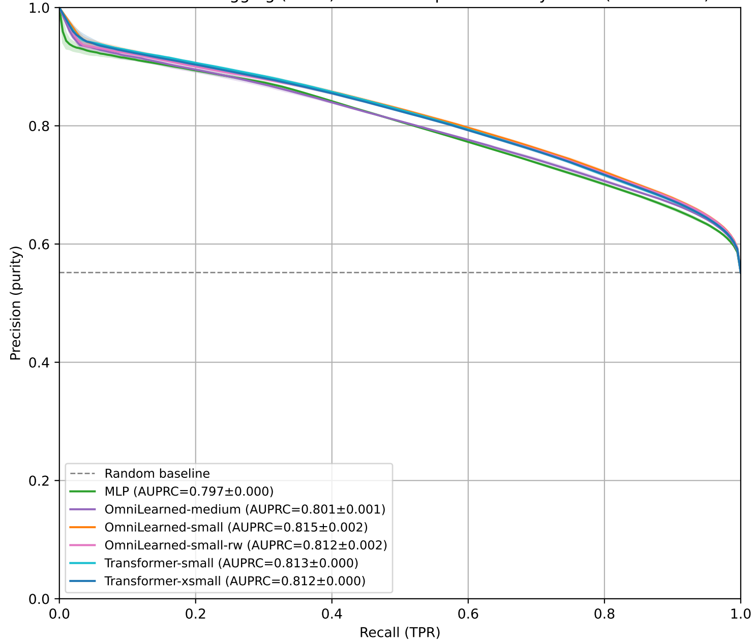
PRC — CCN\pi^\pm tagging ( N \geq 1 ) - Minerva Open Data Playlist 1A (linear scale)
