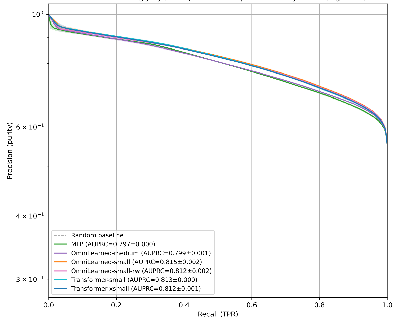
PRC — CCN\pi^\pm tagging ( N \geq 1 ) - Minerva Open Data Playlist 1B (log scale)
