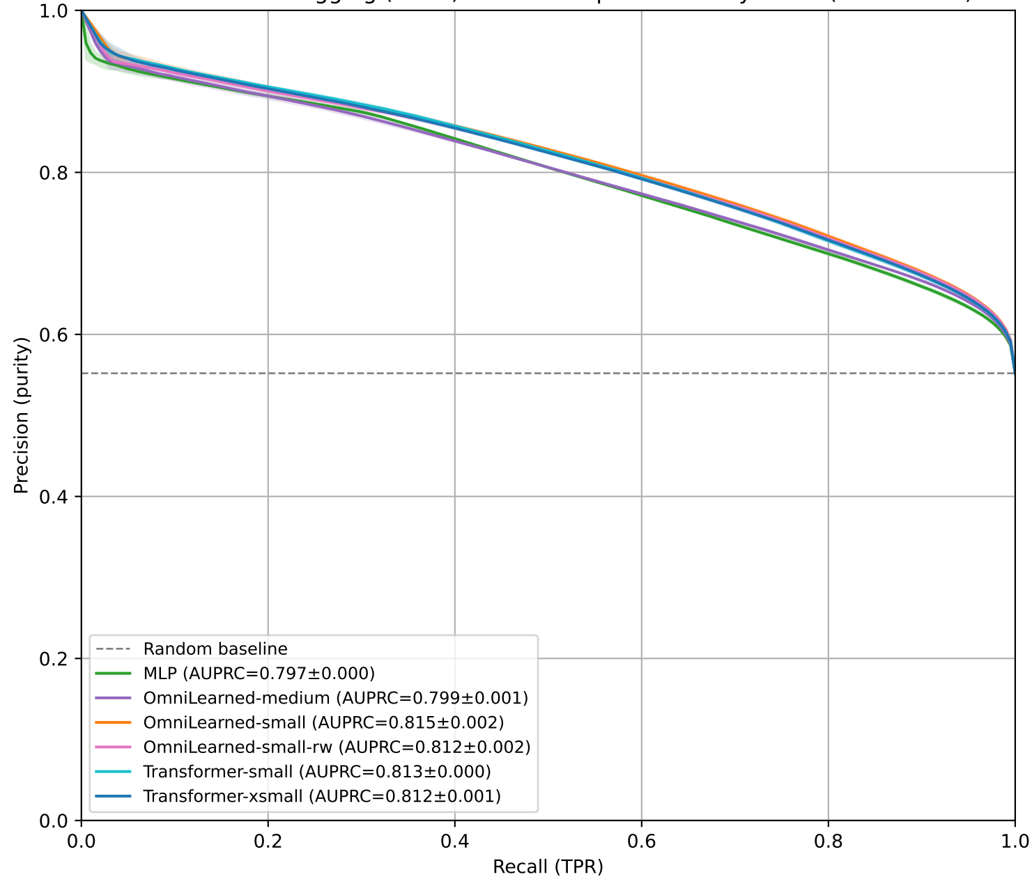
PRC — CCN\pi^\pm tagging ( N \geq 1 ) - Minerva Open Data Playlist 1B (linear scale)
