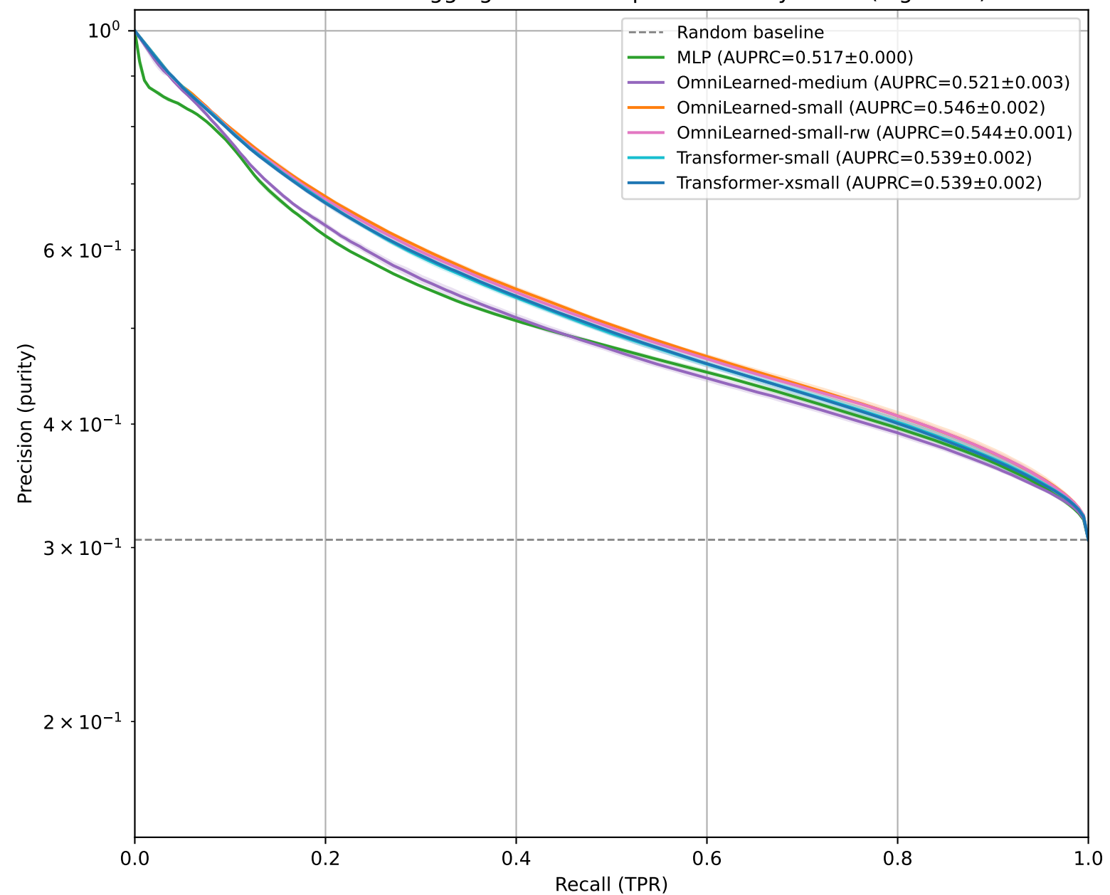
PRC — CC1\pi^\pm tagging - Minerva Open Data Playlist 1A (log scale)
