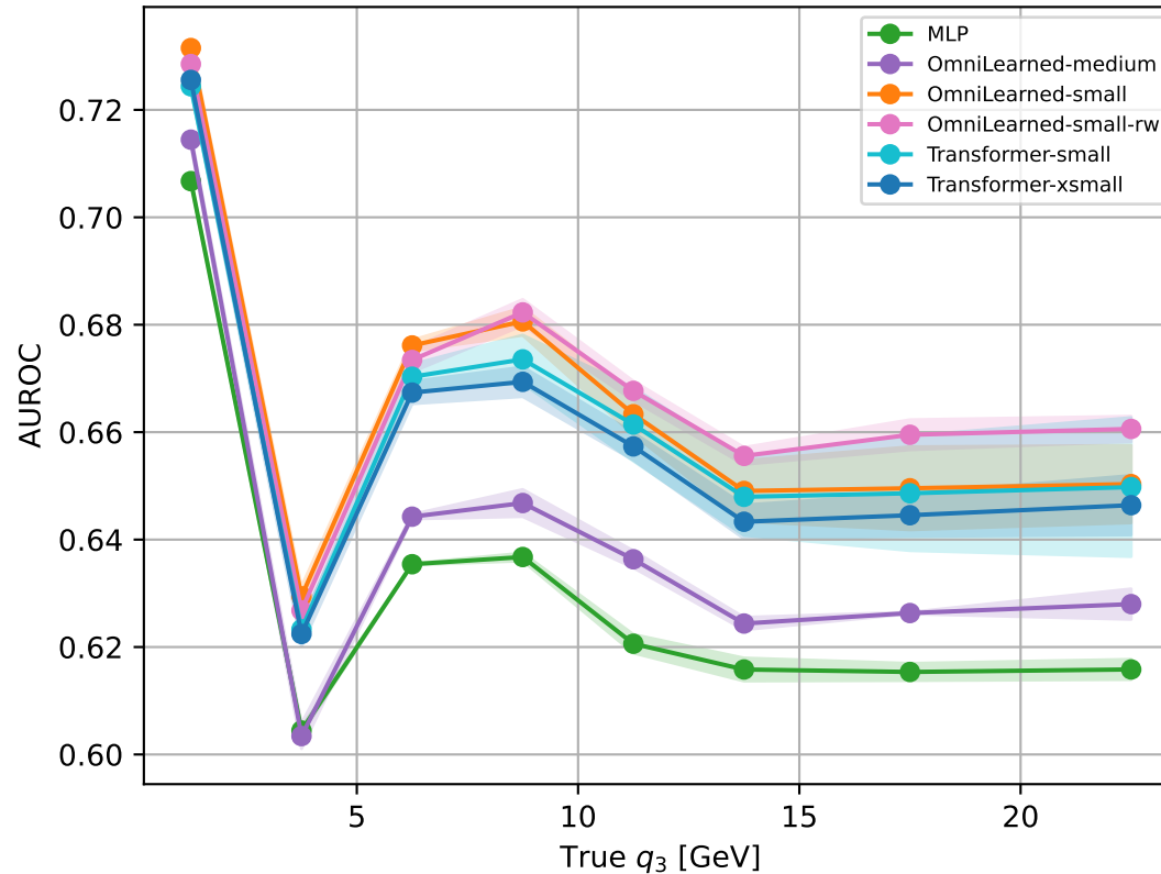
AUROC vs. True q_3
