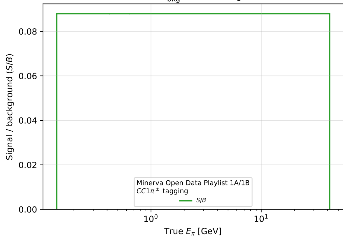
S/B with B = N_{\text{bkg}}^{\text{glob}} (all non-signal, ROC)
