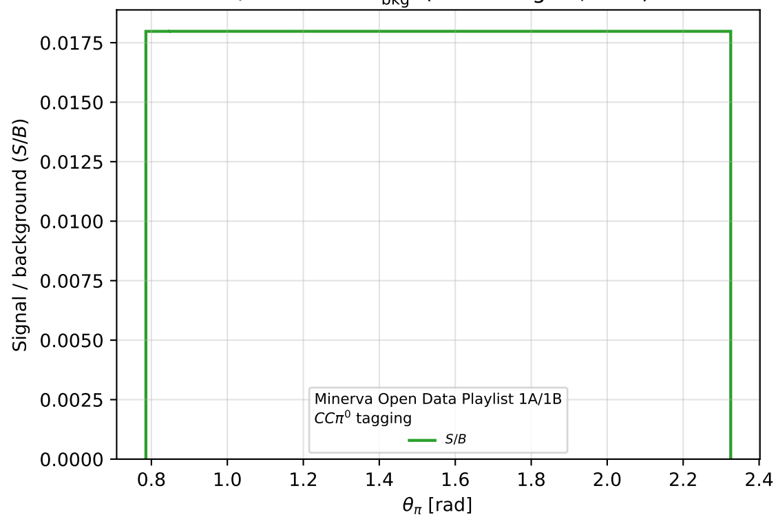
S/B with B = N_{\text{bkg}}^{\text{glob}} (all non-signal, ROC)
