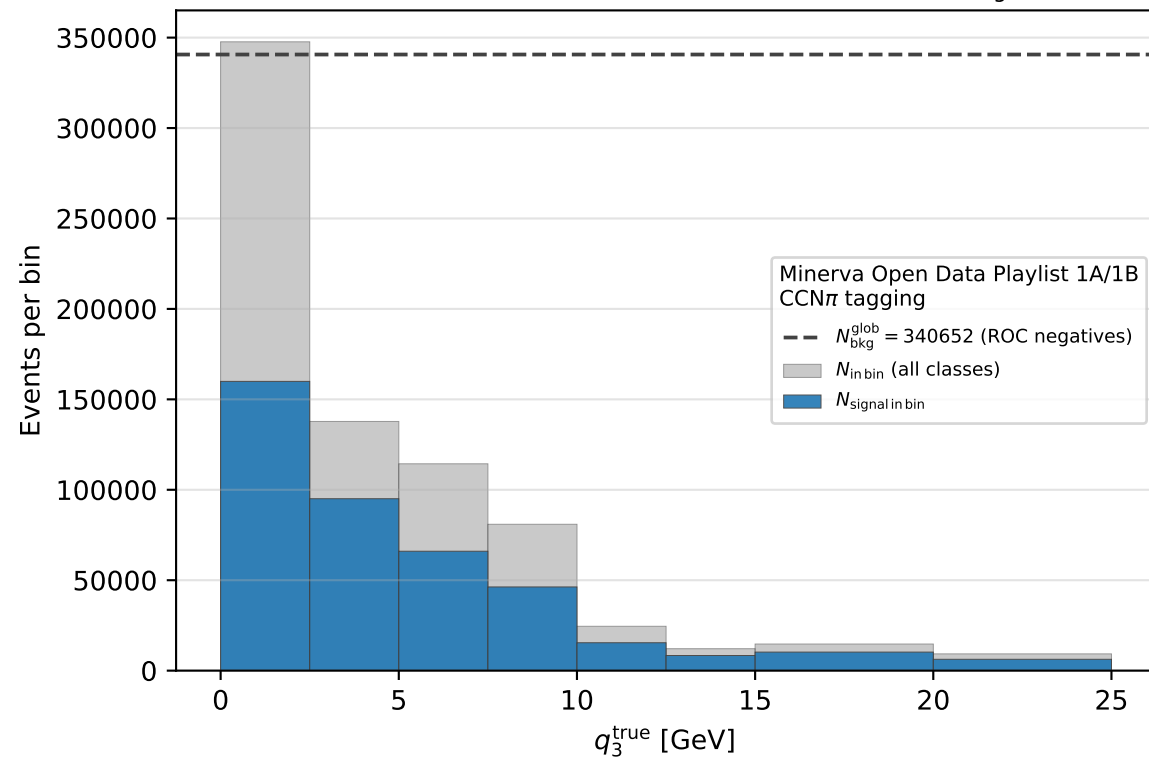
Kinematic bin counts (ROC uses global N_{\text{bkg}} )
