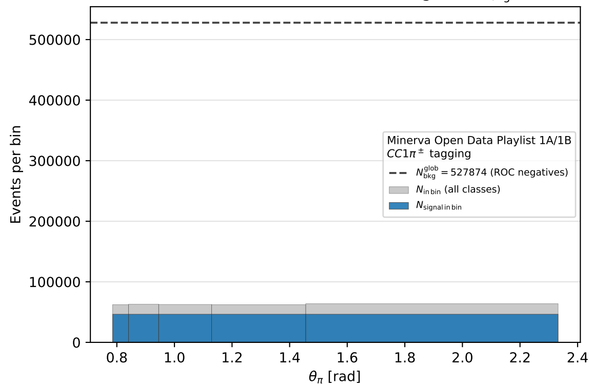
Kinematic bin counts (ROC uses global N_{\text{bkg}} )
