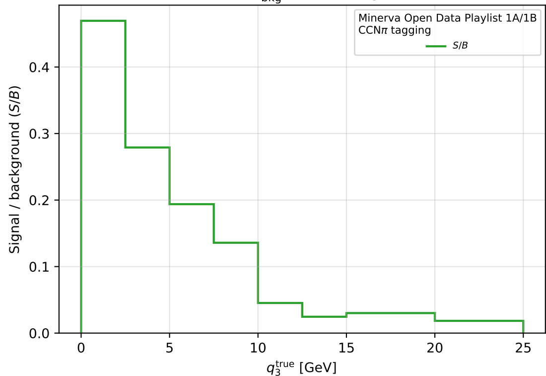
S/B with B = N_{\text{bkg}}^{\text{glob}} (all non-signal, ROC)
