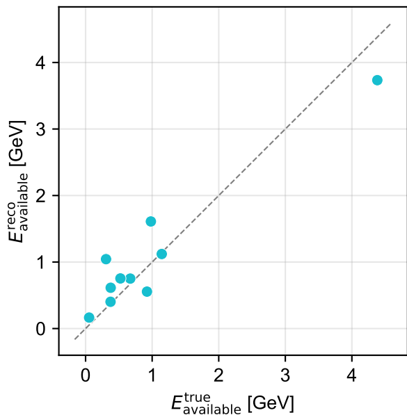
Transformer-small (Log1p)
