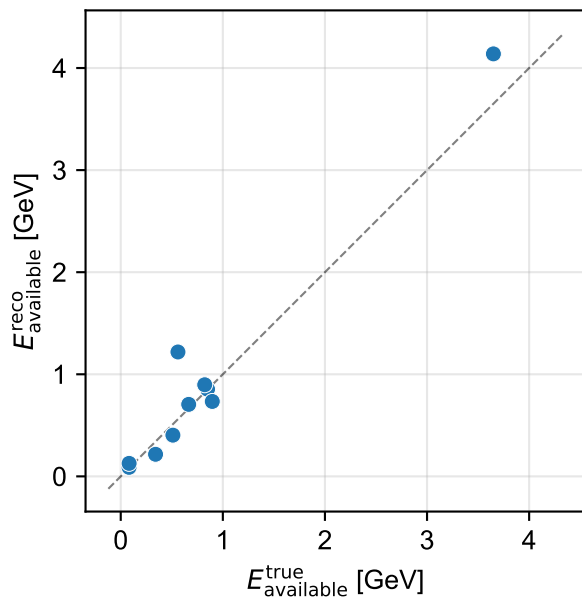
Transformer-xsmall (Log1p)
