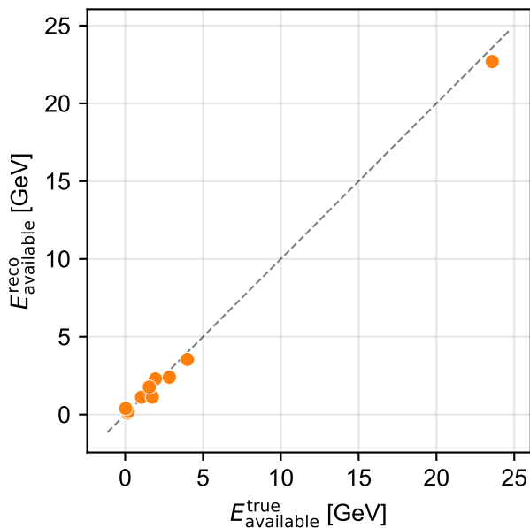
OmniLearned-small (Log1p)
