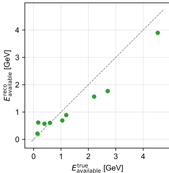
MLP (Log1p)
